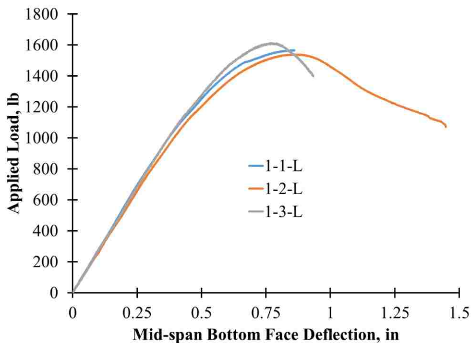
Figure 5.23: Four Point Flexural Test Results of Applied Load vs. Mid-span Bottom Face Deflection for Type 1
