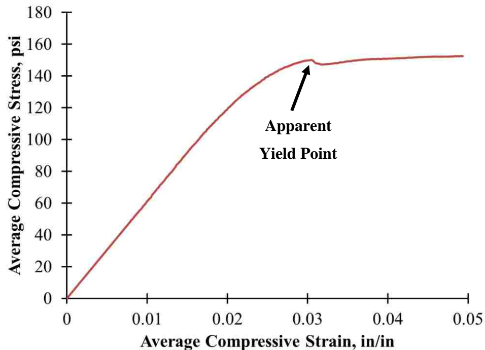
Figure 4.7: Stress vs. Strain at Failure for Flatwise Compression Testing on 1-2-C
