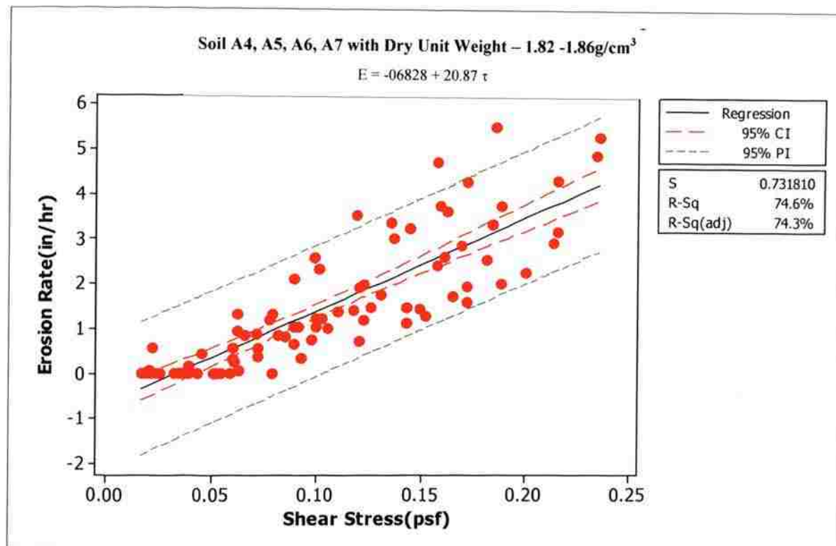
Figure 5.32. Combined Data Plot for Soil A4, A5, A6 and A7 with Similar Dry Unit Weight
