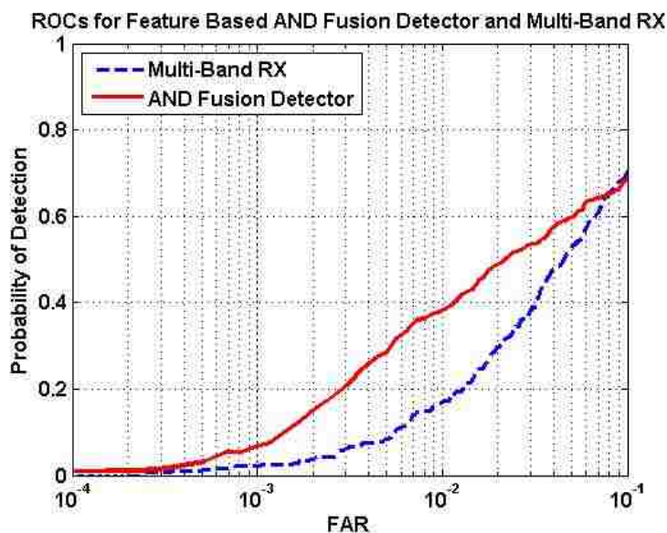
Figure 6.18. Comparison of Detection Performance of the AND Fusion Detector, vis-à-vis Multiband RX Anomaly Detector.
