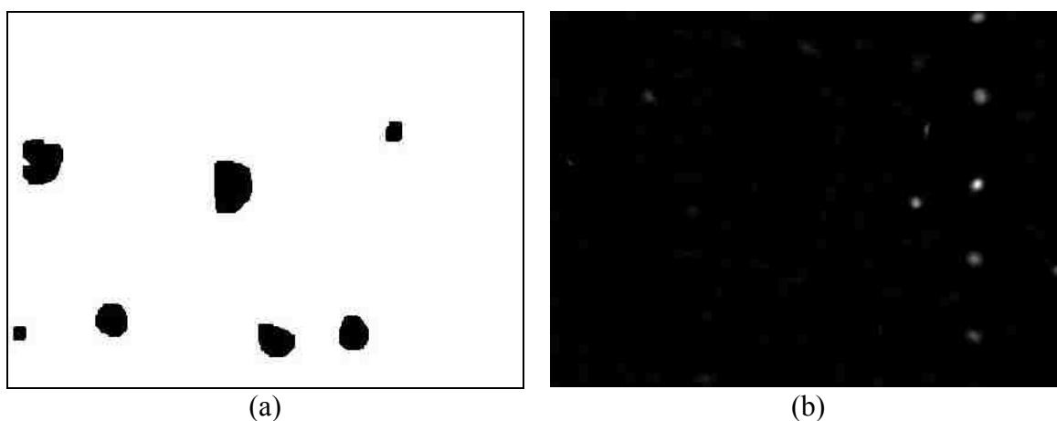
Figure 6.16. Vegetation Based Masking of RX Detector Statistics (a) Mask Image, (b) RX Detector Output with Vegetation Based Masking.
