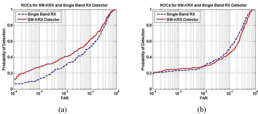
Figure 5.5. Detection Performance of SW-KRX vis-à-vis RX Detector for Green Band Data for Dataset 1 (a) Selected Segments (b) Rest of the Segments.
