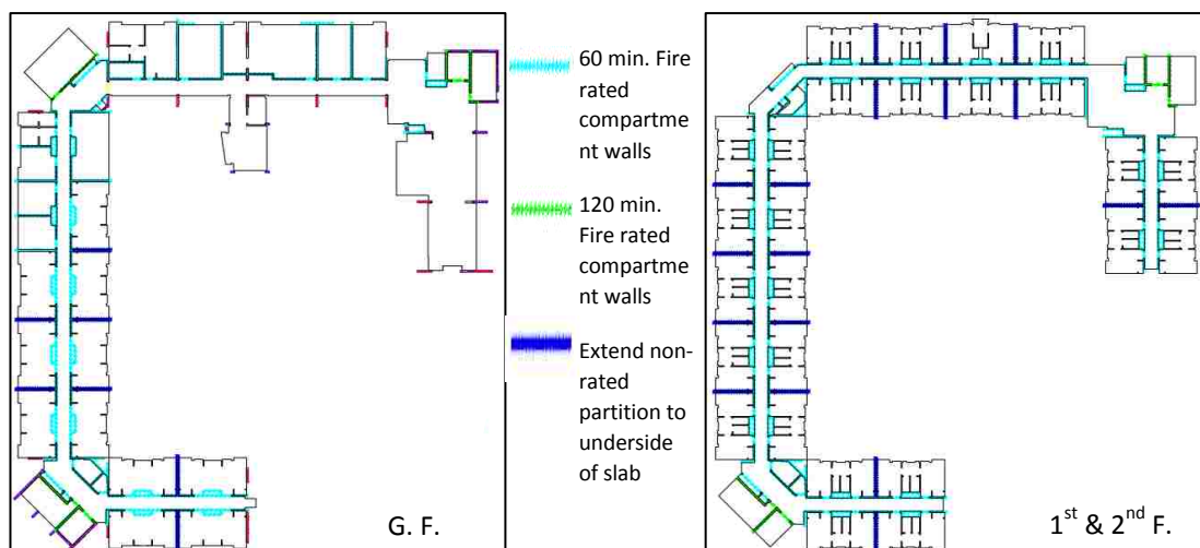
Figure 128: Typical Fire Separation Plans (FSP) in NC hostel
