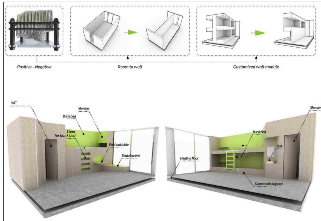
Figure 3: Customized wall module of Bayreuth Youth Hostel in Germany – Source: (“Bayreuth Youth Hostel”, 2015)
