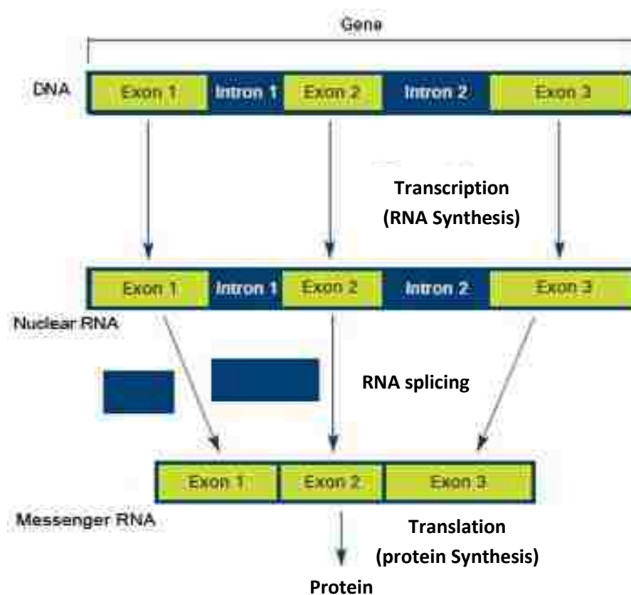
Figure 2: Gene composition [14]
