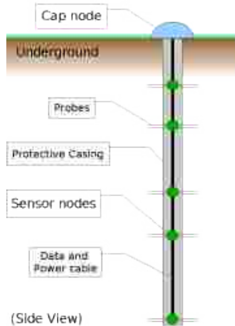
Figure 4.9. Sensor String
