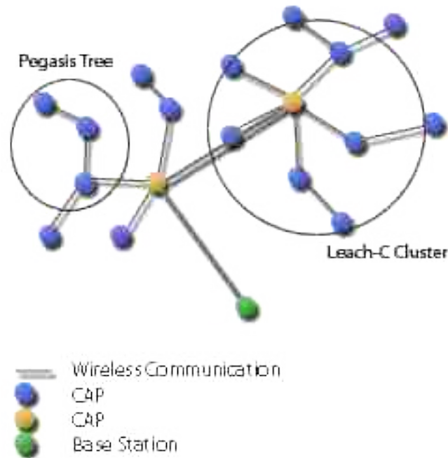
Figure 4.12. Combined Routing Scheme
