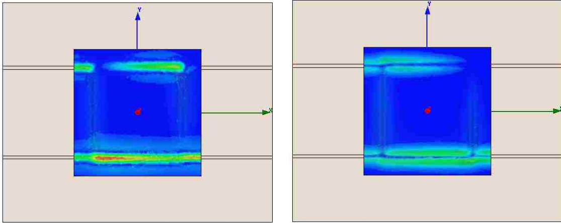
Figure 3.5 |H_y| (left, Units: A/m), |E_y| (right, Units: V/m) simulated at 2 mm above the trace using HFSS
