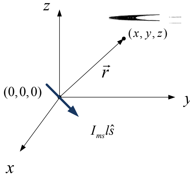
Figure 2.6 A magnetic dipole at the origin
