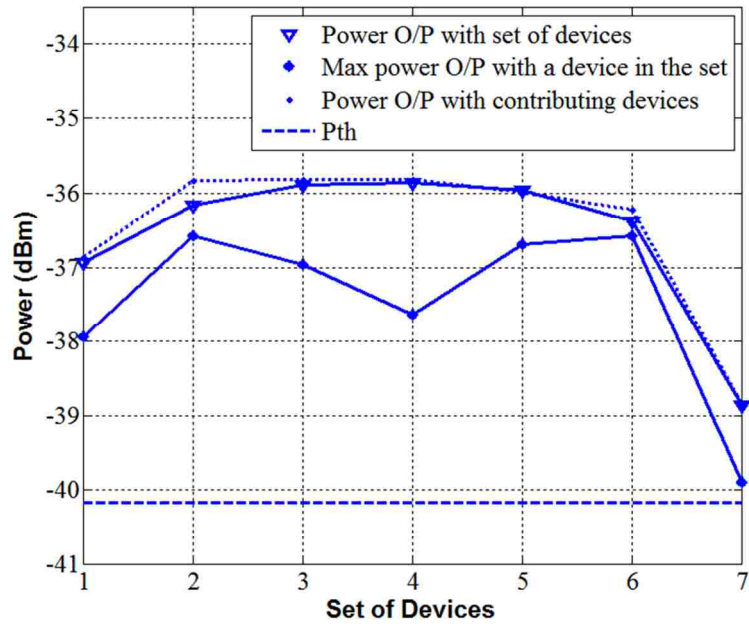
Fig 9. Received power for the best device-sets
