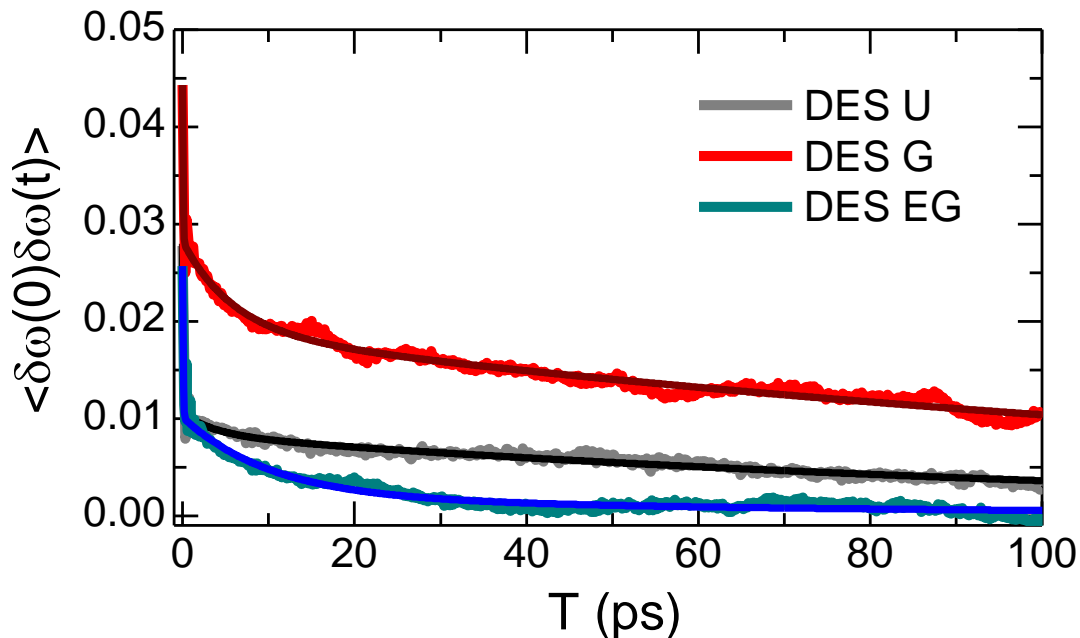
Figure 3.13. Time autocorrelation function of the frequency fluctuations ( \langle \delta\omega(0), \delta\omega(t) \rangle ) obtained from CN distance averaged over 150 fs steps of MD simulations for DES U, DES G, and DES EG.
