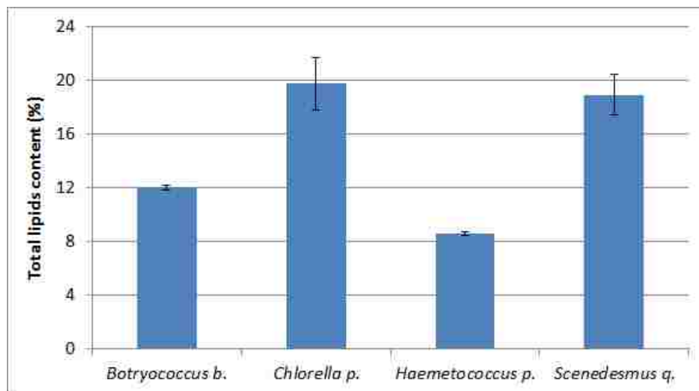
Fig. 1 Extracted total lipids content by using gravimetric method for four green microalgae, Botryococcus b. , Chlorella p. , Haemeticoccus p. , and Scenedesmus q. Three replicate determinations were performed for each sample.
