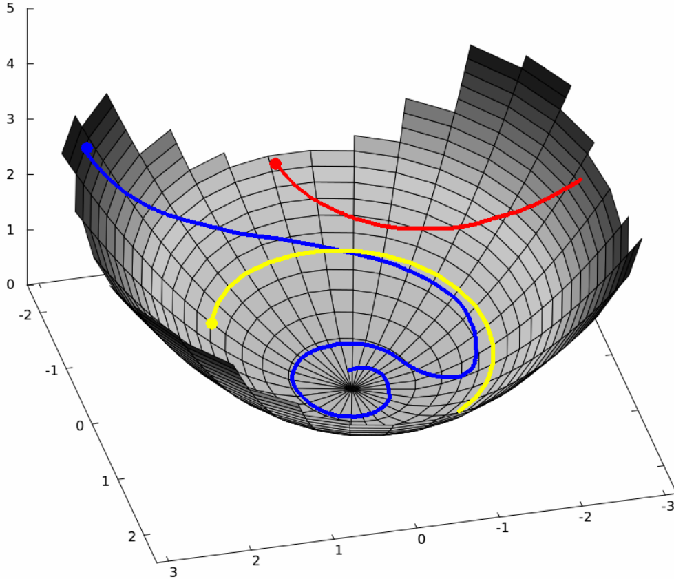
Figure 1.3: A candidate Lyapunov functional with decreasing (blue), non-increasing (yellow), and uncontrolled (red) orbits.
