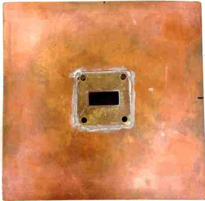
Figure 4.9. Custom-made large flange (152 mm x 152 mm).
