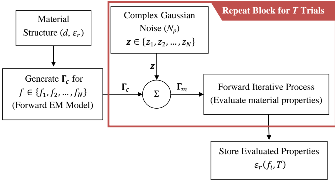
Figure 3.1. Block diagram of simulation to investigate the effect of system noise on the evaluation of material properties.
