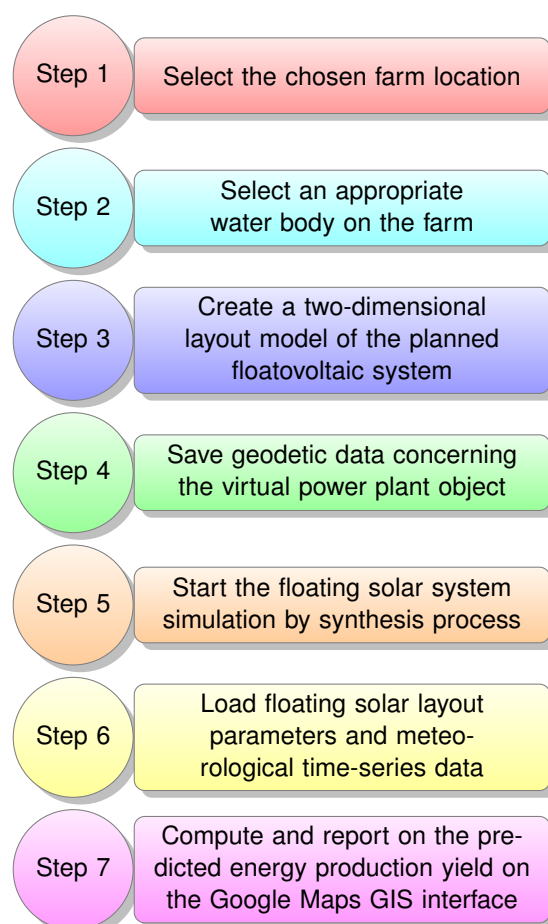
Figure 4.9: Experimental steps for determining the energy yield profile for floating solar systems in a case-based analysis scenario.
