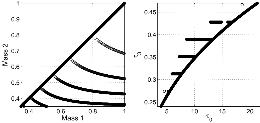
Figure 2.4: Template banks are chosen to cover a parameter space (e.g. component masses between 0.35M_{\odot} and 1M_{\odot} ) such that a real signal that falls in-between the discrete template spacing would still produce > 1-\delta of a perfect match SNR. The resulting spacing is a function of mass, left. It is possible to find a coordinate transformation that make the spacing nearly rectilinear, right. The coordinates are \tau_0 \propto m_1 m_2 m^{-5/3} and \tau_3 \propto m_1 m_2 m^{-2/3} .
