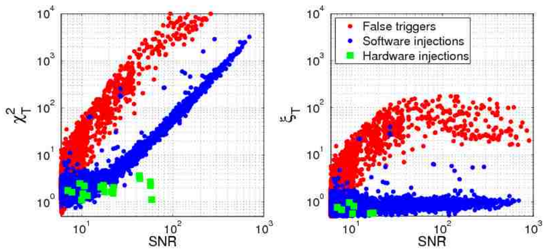
Figure 6.8: Left: SNR \chi_T^2 scatter plot of L1 triggers. Right: SNR \xi_T scatter plot of L1 triggers.
