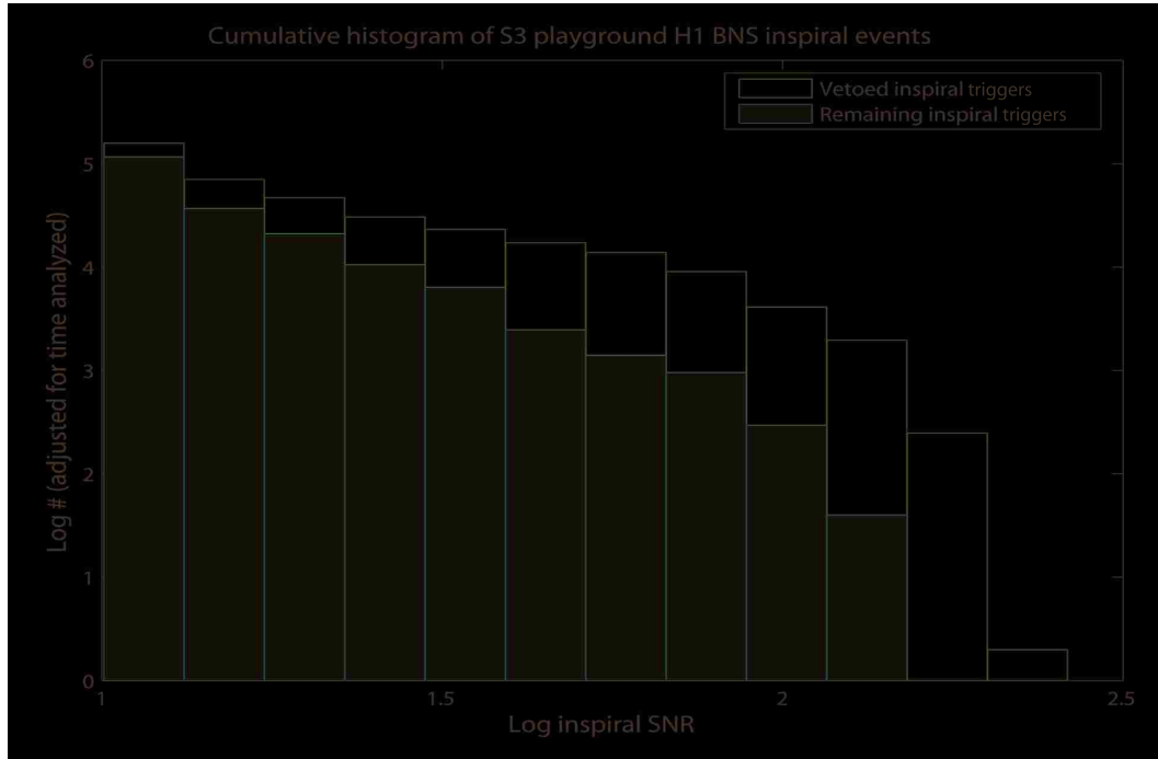
Figure 5.5: A cumulative histogram of the number of BNS triggers in the S3 playground data from the H1 detector versus the threshold on the BNS trigger SNR (upper histogram). Many of the high SNR BNS triggers are coincident with ASI glitches, with values of \kappa consistent with noise glitches, and can be vetoed; unvetoed triggers are in the lower histogram.
