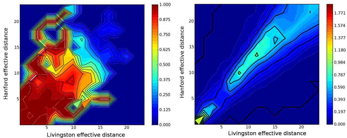
Figure 2.16: Left: S4 PBH efficiency vs effective distance in Hanford and Livingston sites. The efficiency depends on mass and has been normalized to a 1.4, 1.4 M_{\odot} system in this plot (we use this as a canonical mass for the PBH and BNS searches in order to make direct comparisons that are less waveform dependent). The product of the efficiency and blue light luminosity obtained from a galaxy catalog is integrated over effective distance in order to obtain the cumulative luminosity C_L . Right: S4 PBH luminosity density vs effective distance. The distance and blue light luminosity from a galaxy catalog (34) is binned up into effective distance bins for the Hanford and Livingston detectors. This luminosity density is integrated with the efficiency to produce the cumulative blue luminosity available to the search C_L .
