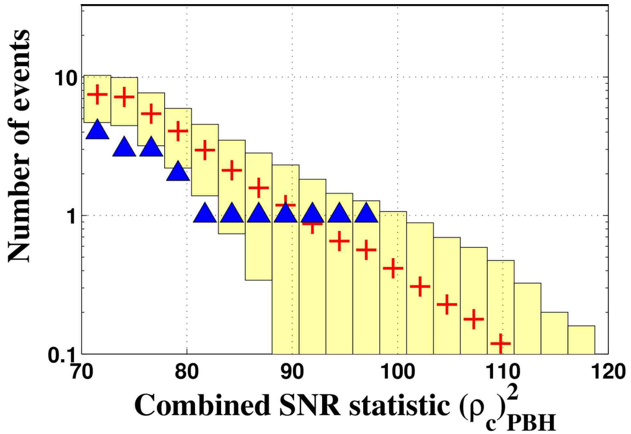
Figure 2.15: Cumulative histogram of candidate events for the S4 PBH search after category 2 vetoes. The candidate events are consistent with the false triggers found by performing time shifts. No plausible gravitational-wave candidates were found.
