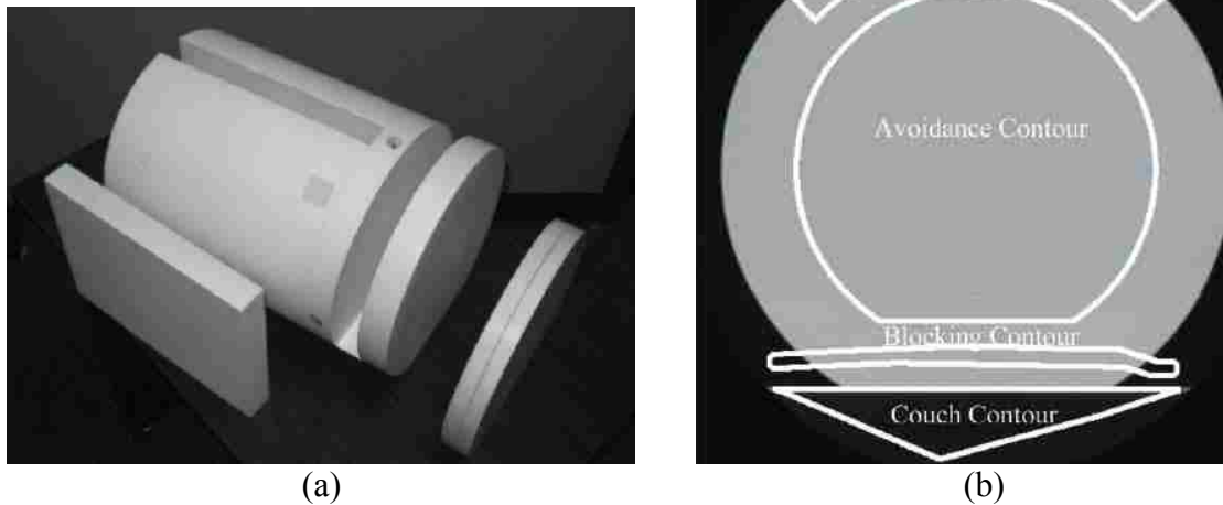
Figure 1.4. Pictures of (a) 13.5-cm radius by 37.4-cm length white opaque high-impact polystyrene cylindrical phantom is depicted with axial and sagittal film cassettes removed from the phantom and (b) TomoTherapy treatment planning image showing the 2 cm thick PTV, avoidance, blocking, and couch contours. (Cheek et al 2006)
