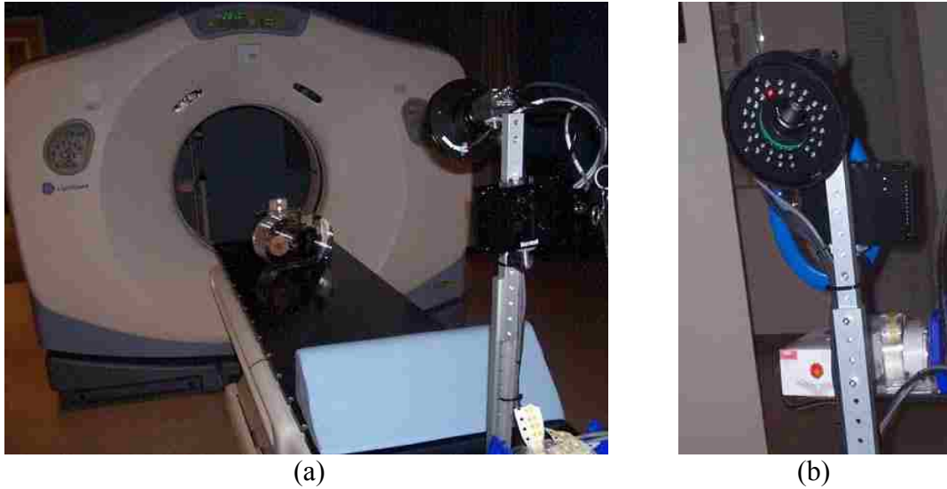
Figure 1.8. Pictures of (a) RPM respiratory gating system and (b) infrared emitting diodes surrounding a camera
