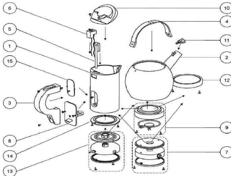
Figure 2.8 Parts used in the kettle product family (AlGeddawy and ElMaraghy 2010a)
