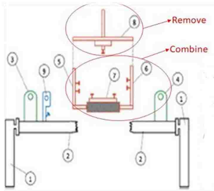
Figure 4.6: Side support, bottom support, and side support 2 (combined), Top support (removed) are circled
