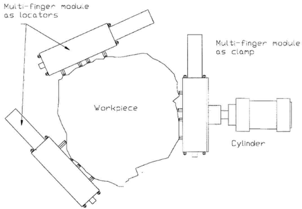
Figure 2.3: CNC modular fixture for assembly presented by Chan and Lin (1996)
