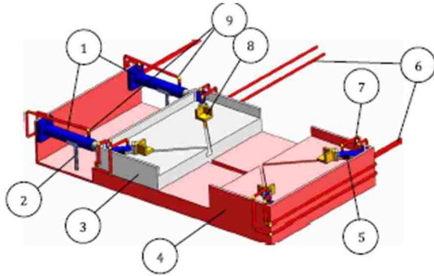
Figure 3.4: Isometric view of the reconfigurable assembly fixture to show the components presented in table 3.1 adopted by Olayinka
