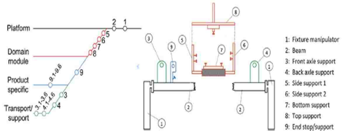
Figure 4.3: Cladistics analysis of the new proposed fixture architecture Adopted by Bejleggaard et al. (2018)
