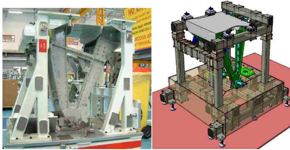
Figure 2.6: a. Existing Conventional A380 Rib 17 Subassembly fixture (courtesy of Airbus UK) b. The modular and configurable version of the A380 Sub-assembly fixture by Helgossan et al. (2010)
