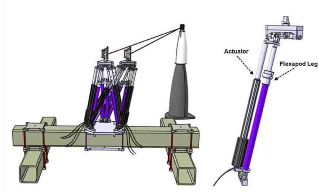
Figure 2.5: Flexapod with motor-driven actuator attached to the legs. An outer measuring system ensures accuracy presented by Jonsson et al. (2010)
