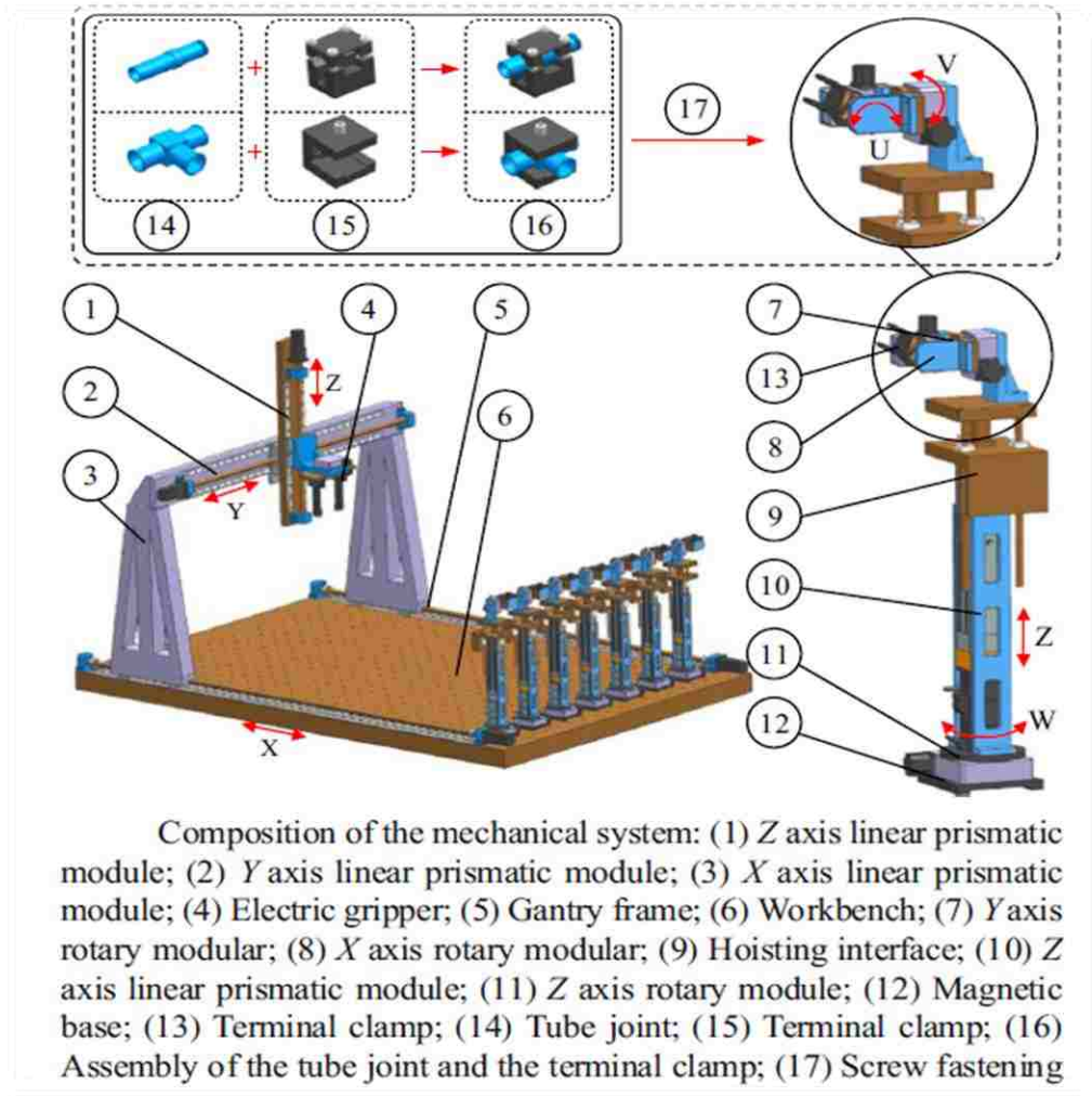
Figure 3.6: Composition of the mechanical system by Fan et al. (2018)
