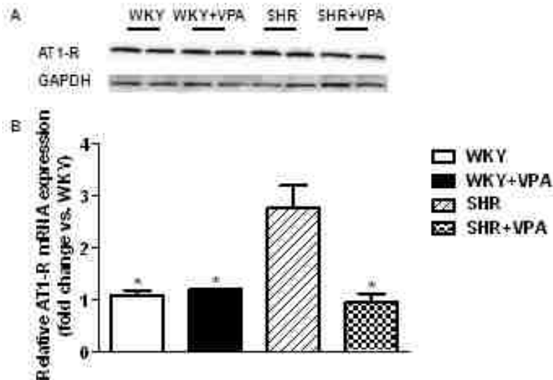
Figure 3.4. Effect of VPA on AT 1 R mRNA and protein expression. Untreated SHR rats showed higher mRNA (B) and protein expression (A) levels of the AT 1 R in the LV when compared to WKY controls. SHR+VPA attenuated this increase. Western blot protein expression bands were normalized to GAPDH. n=7-8 in each group, * p<0.05 vs SHR.
