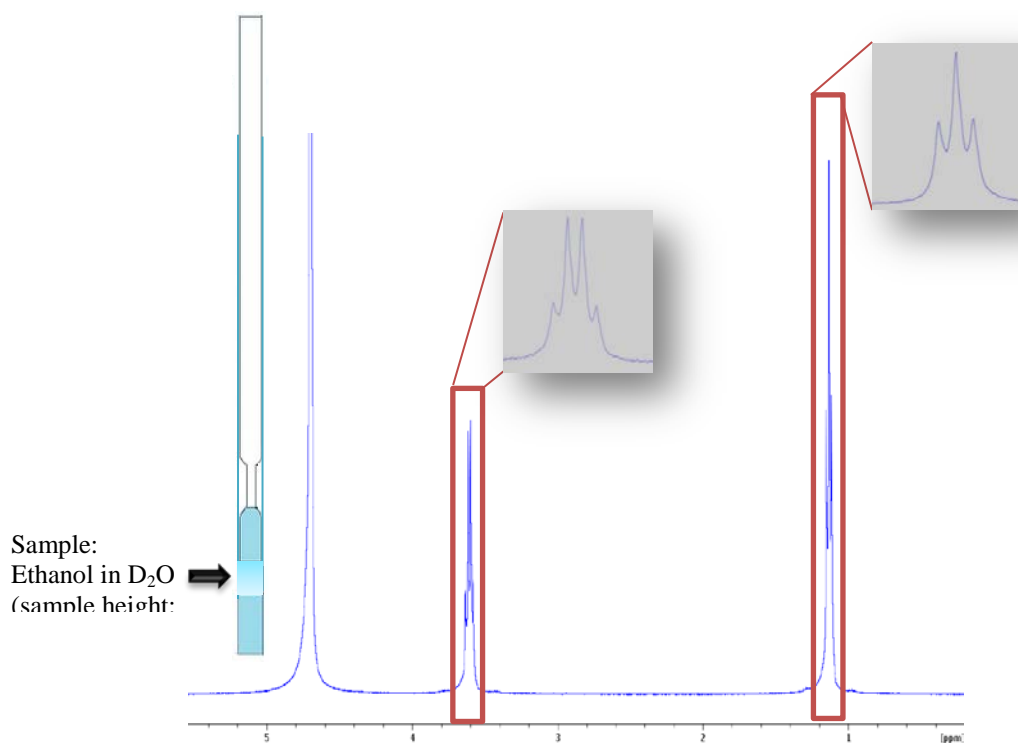
Figure 2.12. ^1\text{H} NMR spectrum of a 4.8 Vol% ethanol (94%, commercial grade) \text{D}_2\text{O} (99.8% D) solution in a susceptibility-matched Shigemi tube.
