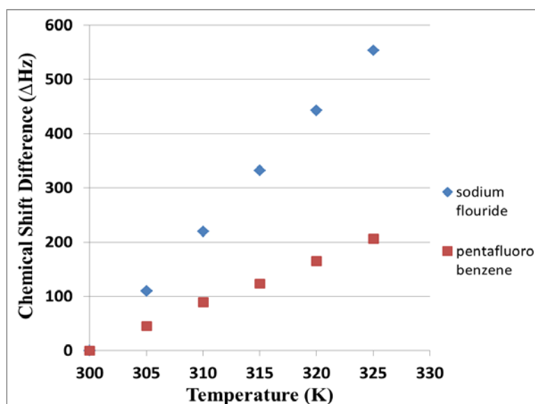
Figure 2.2. 19 F chemical shift changes of pentafluorobenzene (C 6 F 5 H) and sodium fluoride (NaF) signals in aqueous solution at temperature between 300 and 325K.
