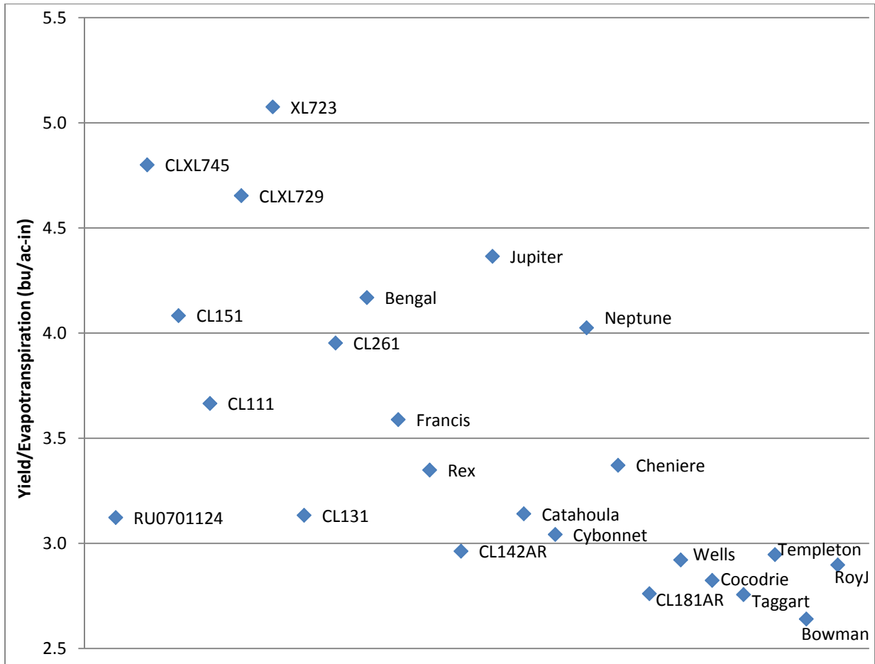
Figure 18. Yield/Evapotranspiration (bu/ac-in) Ratio for Rice Varieties at the Stuttgart ARPT Station in 2010
