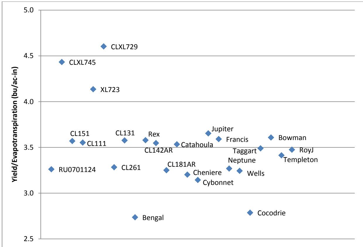
Figure 22. Yield/Evapotranspiration (bu/ac-in) Ratio for Rice Varieties at the Newport ARPT Station in 2010
