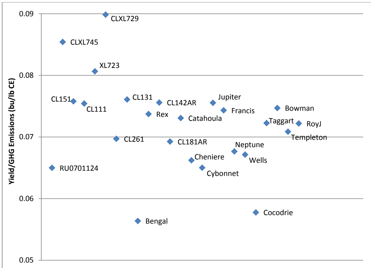
Figure 28. Yield/GHG Emissions (bu/lb CE) Ratio for Rice Varieties at the Colt ARPT Station in 2010
