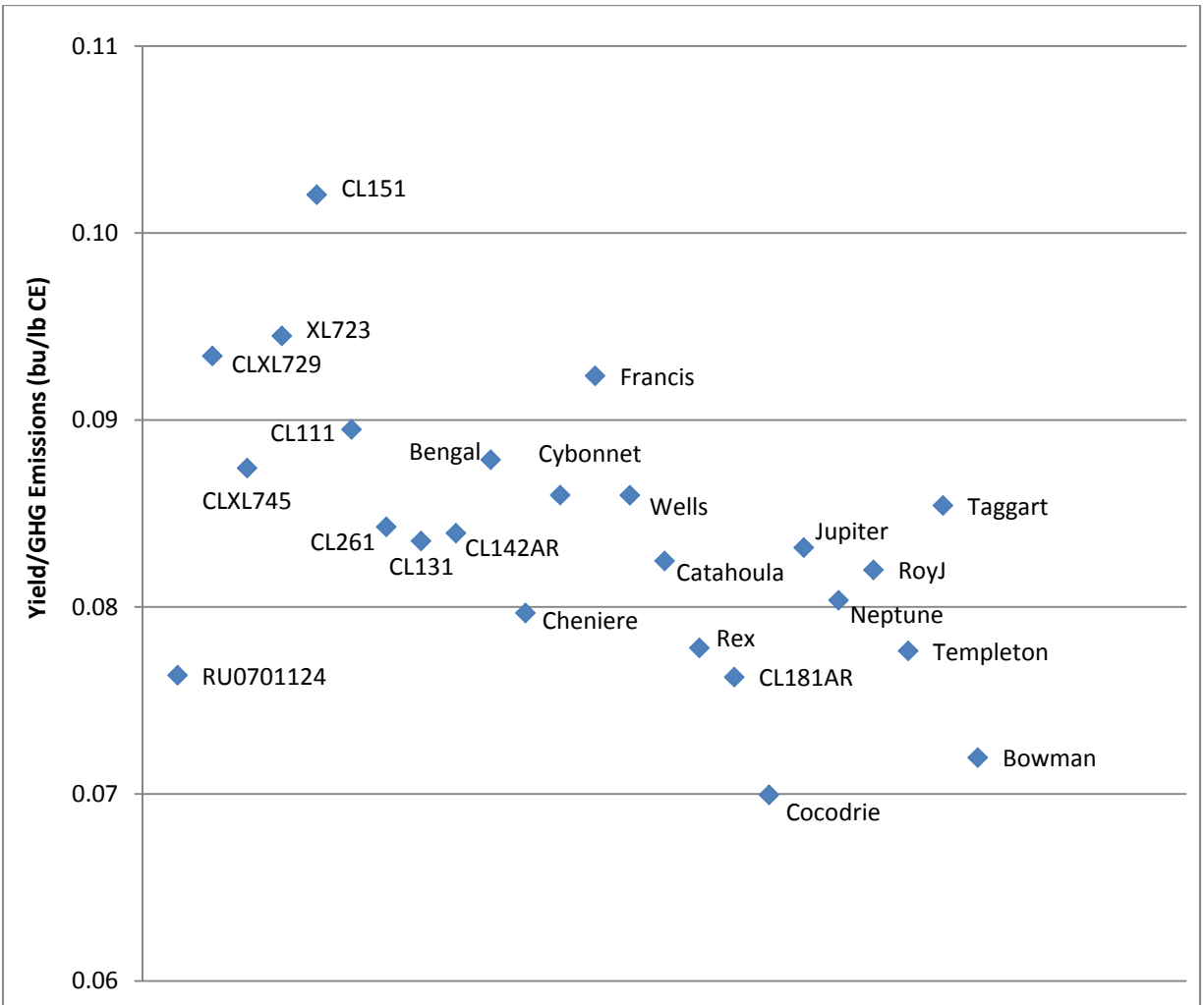
Figure 29. Yield/GHG Emissions (bu/lb CE) Ratio for Rice Varieties at the Coring ARPT Station in 2010
