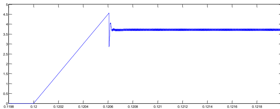
Figure 4.60 Phase-2's error voltage in converter-2 for T_u=500 \mu s
