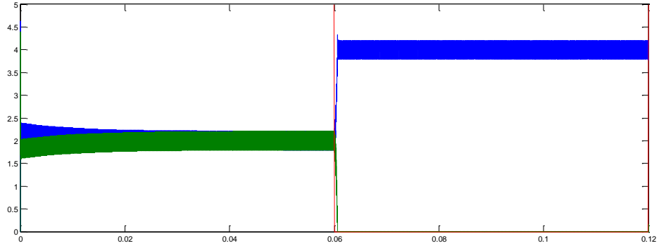
Figure 4.14 Phase current in converter-1 for T_d=500 \mu s
