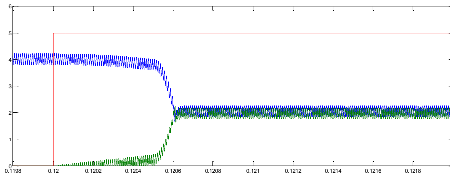
Figure 4.57 Zoomed in phase currents in converter-2 for T_u=500 \mu\text{s}
