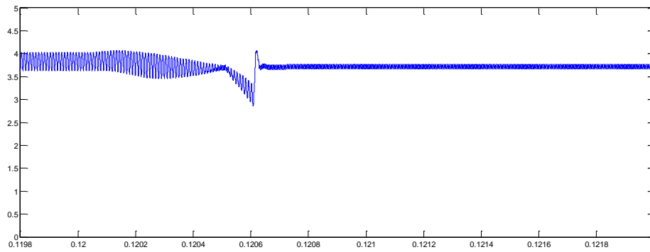
Figure 4.59 Phase-1's error voltage in converter-2 for T_u=500 \mu s
