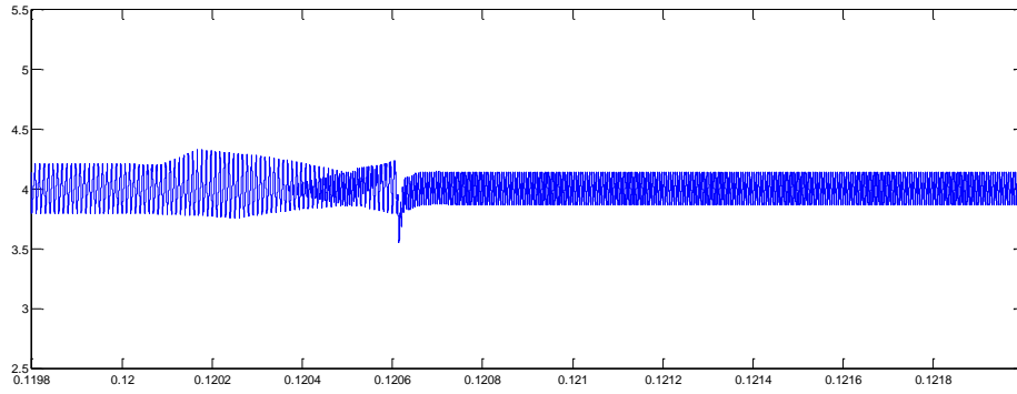
Figure 4.58 Total current in converter-2 for T_u=500 \mu s
