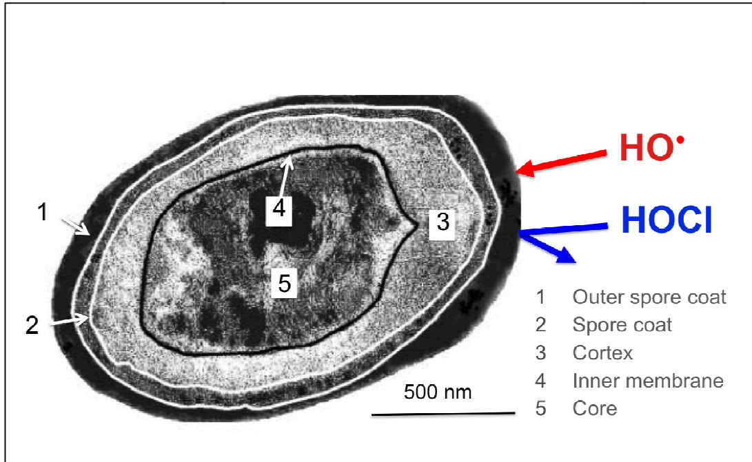
Figure 3.15: Schematic of extracellular HO^\bullet and FAC attack. (Electron micrograph image adapted from Driks et al. 1999 (86)).
