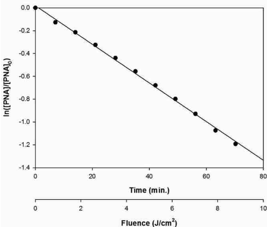
Fig 3.2: PNA loss versus time and fluence. Conditions: [PNA] = 50 \mu M, [Pyridine] = 10 mM, Temperature = 25 ^{\circ} C, and simulated sunlight with DM and AAF. Regression fit: y = -0.017x + 0.0188 , R^2 = 0.998 .
