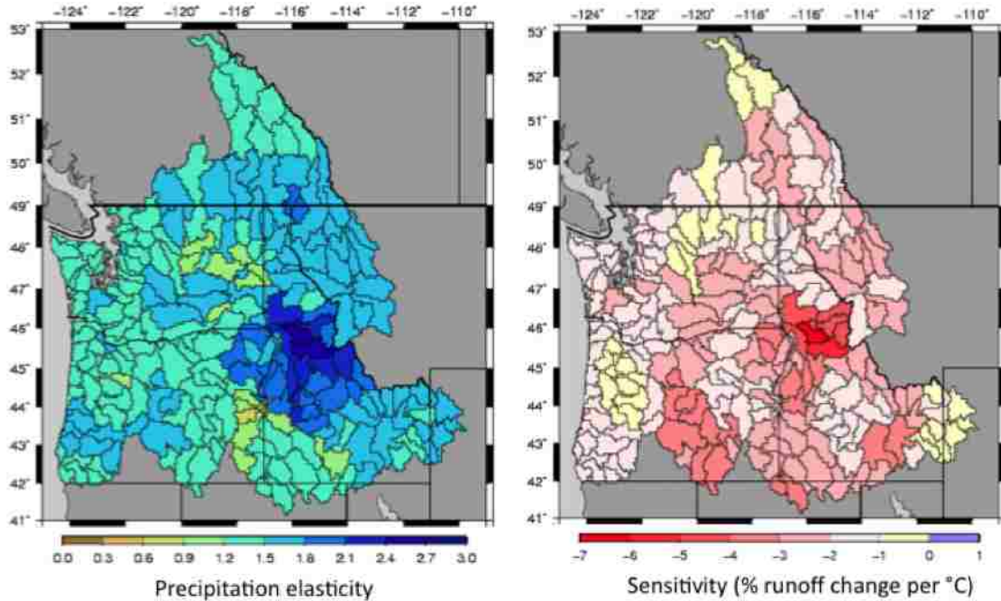
FIG 4.5 Watershed scale annual precipitation elasticities ( \epsilon ) and temperature sensitivities ( S ). Annual responses (percent) to annually applied change (percent precipitation change or ^{\circ}\text{C} warming)
