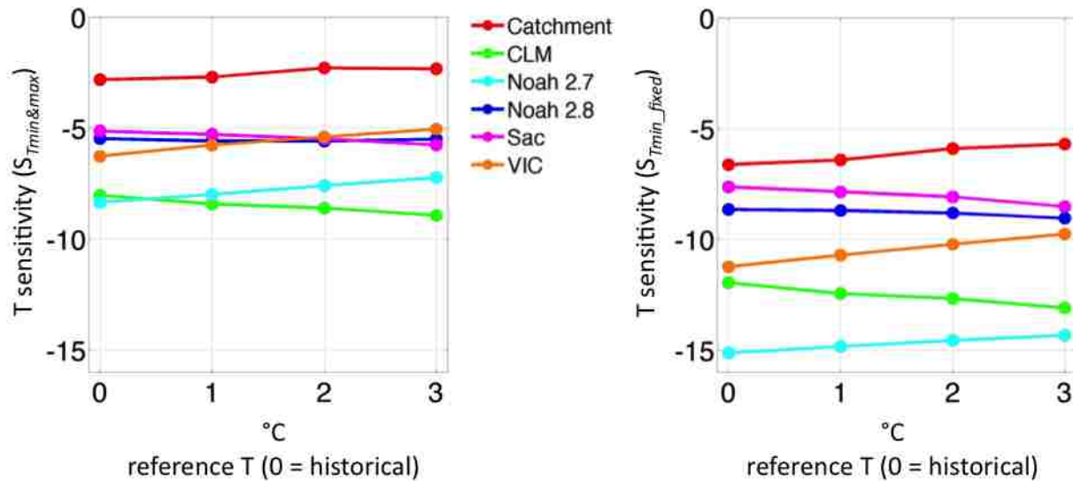
FIG 2.8 Temperature sensitivities (S) at Lees Ferry. Values on y-axis are S from Eq. 2.2 by increasing both T_{\min} and T_{\max} by \Delta (left panel) and by fixing T_{\min} and increasing T_{\max} by 2\Delta (right panel) at historical 1°C, 2°C, and 3°C reference climates, \Delta=0.1^\circ\text{C} .
