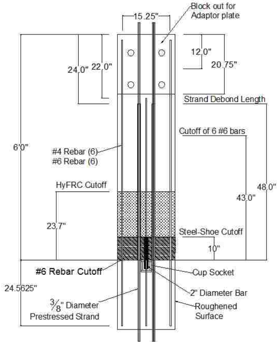
Figure 2.3 Elevation view of the specimen PreT-SF-ROCK-HyFRC.
