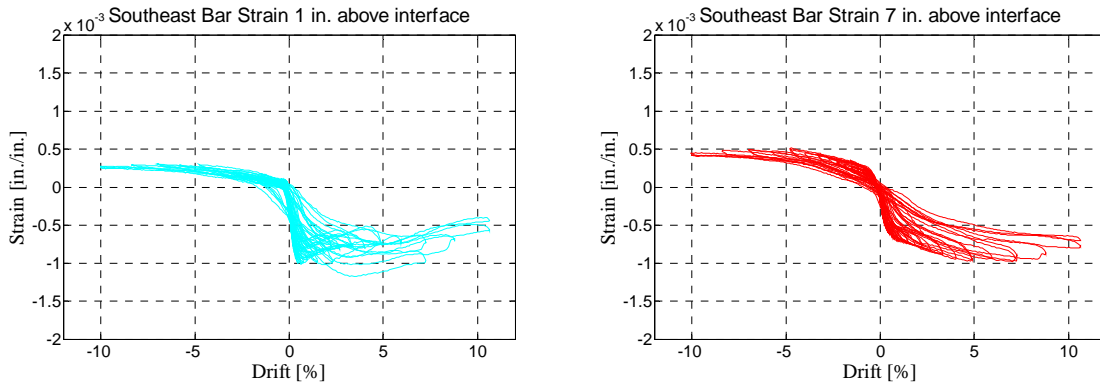
Figure 5.33 Strain vs. drift in Southeast No 6 Bar, PreT-SF-ROCK-HyFRC.
