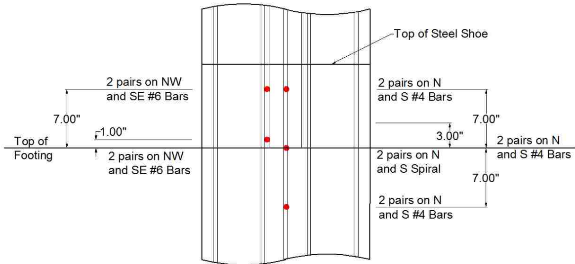
Figure 3.4 Column elevation view of 3-wire strain gauge placements.
