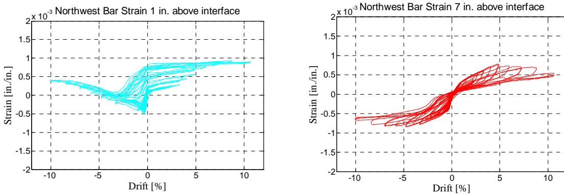
Figure 5.34 Strain vs. drift in Northwest No 6 Bar, PreT-SF-ROCK-HyFRC.
