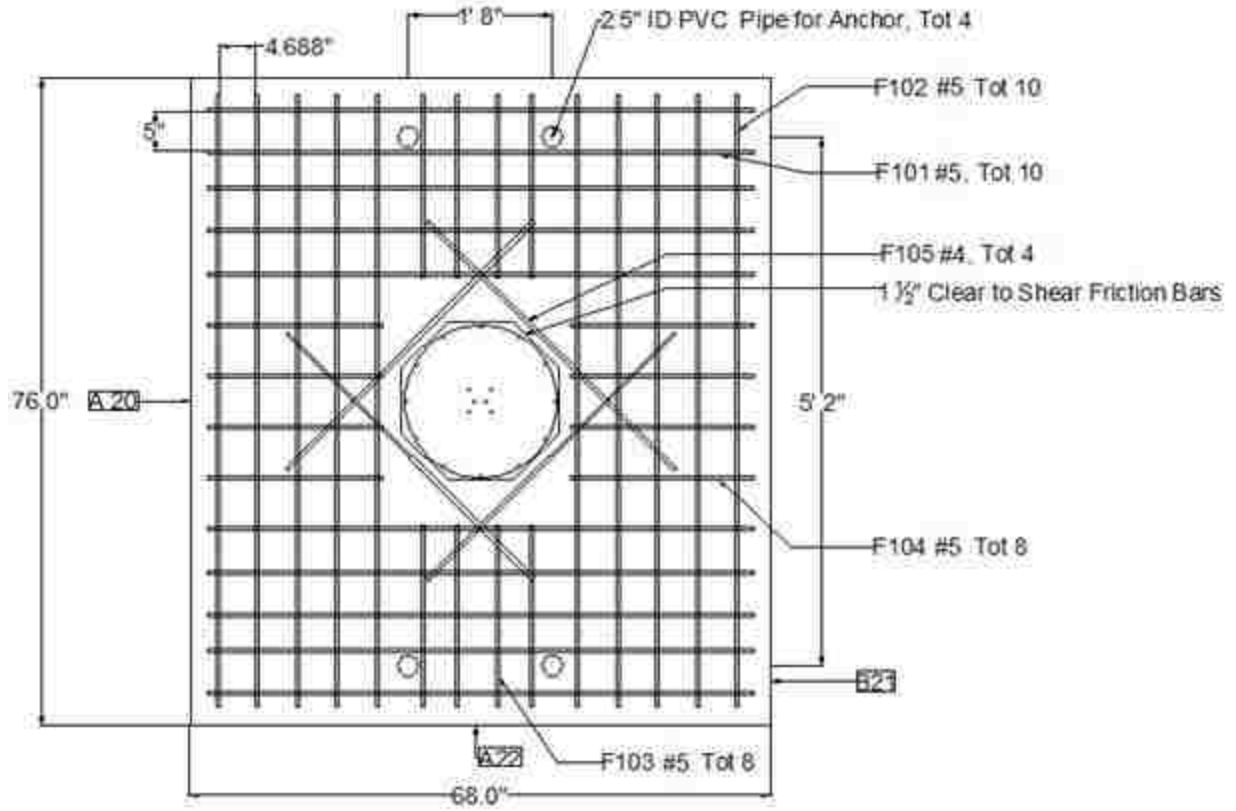
Figure B.7 Footing bottom mat.
