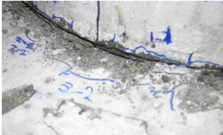
Figure 4.6 South view of PreT-SF-ROCK showing the fillet spalling of the footing induced by the rocking action of the steel shoe.
