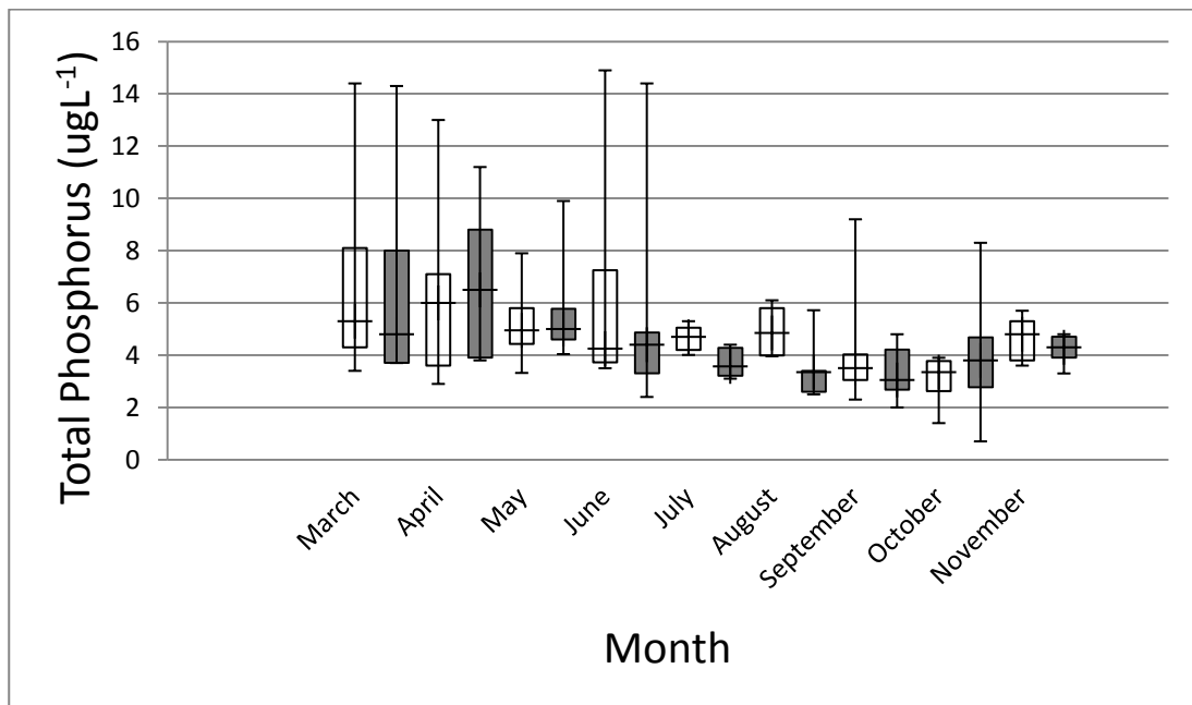
Figure 5: Total phosphorus concentrations in Lake Chaplain, 2005-2011 (Grey bars 1.5m, Clear bars ca.18m). Orthophosphate levels are barely detectable in Lake Chaplain.
