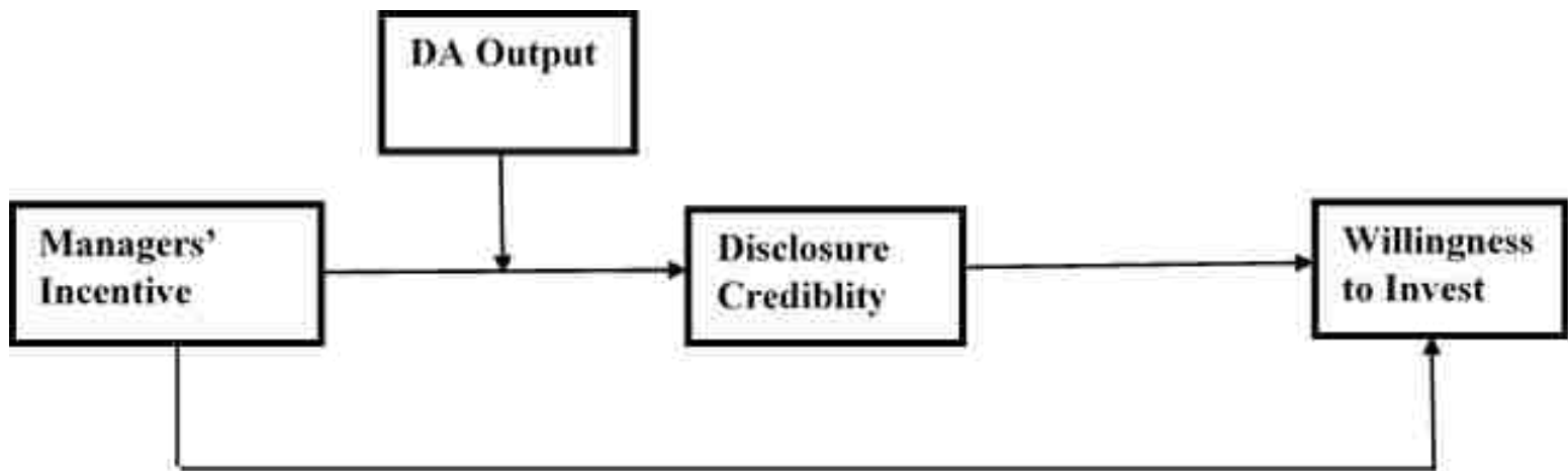
Figure 3: Theoretical Model
