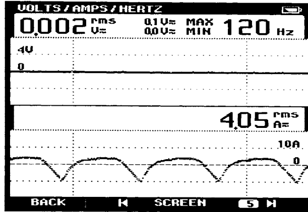
Figure 5.2. Fluke Probe Current Measurement at Sundown on Nov. 17, 2006
