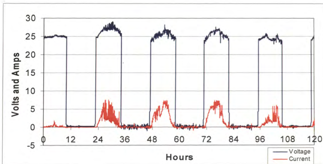
Fluorescent light test results, showing the voltage and current values collected by the panel, from February 13 – 17, 2007.
