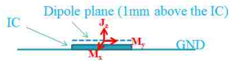
Figure 3.5 \mathbf{J}_z , \mathbf{M}_x and \mathbf{M}_y dipoles are chose to predict far-field
