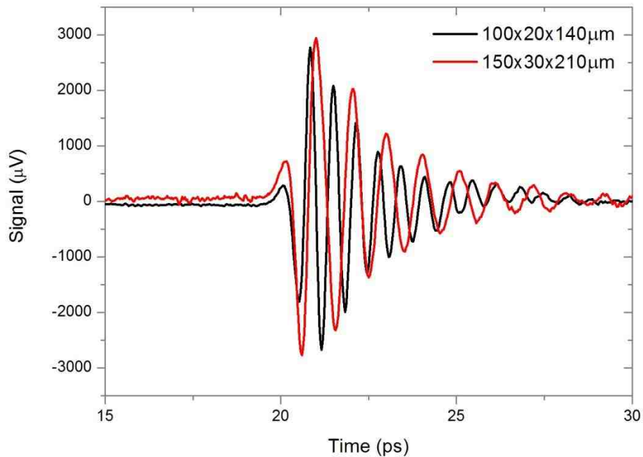
Figure 5.5: Time-domain response to a broadband THz-TDS pulse.
