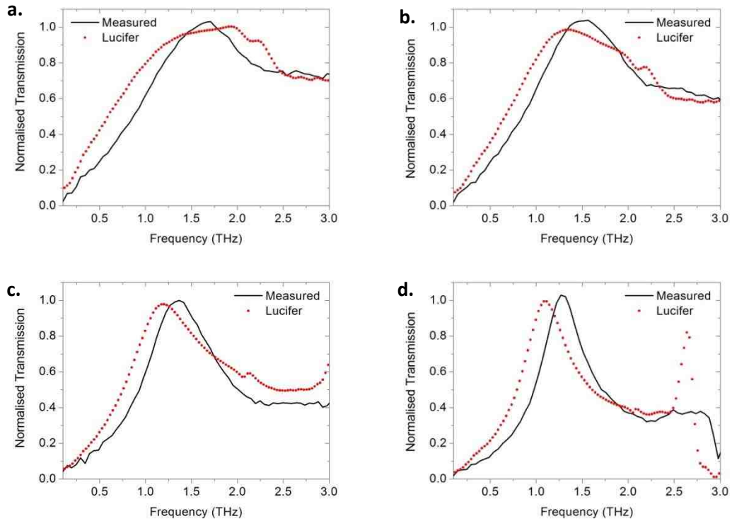
Figure 5.18: Normalised THz-TDS transmission of 125 \times 25\ \mu\text{m} aperture arrays with fixed 135\ \mu\text{m} y direction periodicity and varied x direction periodic spacing compared to Lucifer FDTD simulations. X direction periodic spacing; a. 35\ \mu\text{m} , b. 50\ \mu\text{m} , c. 75\ \mu\text{m} , d. 100\ \mu\text{m} .
