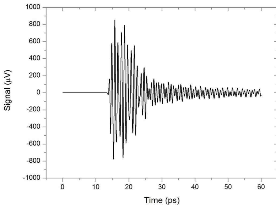
Figure 7.3: Time-domain response of double 150 \times 30 \mu\text{m} aperture array with a 210 \mu\text{m} square lattice separated by 250 \mu\text{m} of free space.
