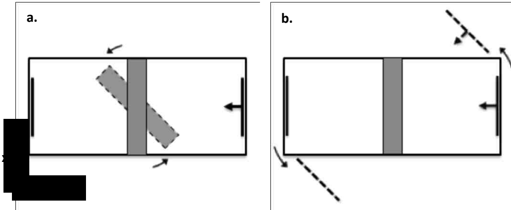
Figure 4.5: FDTD simulation domain for a. Tilted PEC array and b. Rotated monitor and source.
