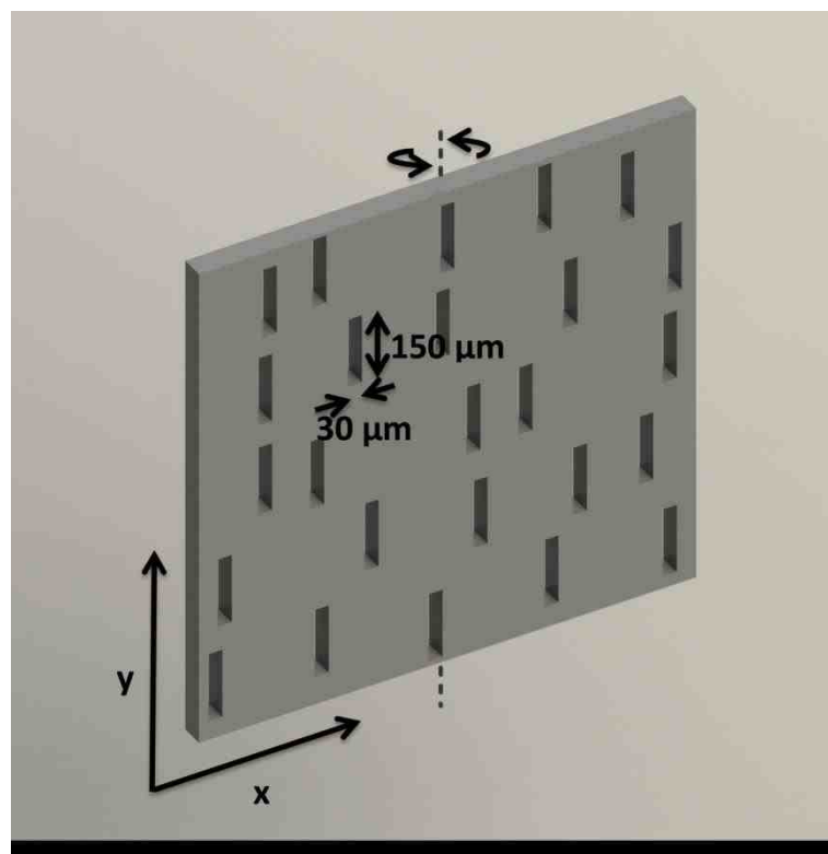
Figure 6.8: Repeating pattern of 5 \times 5 randomly located 150 \times 30 \mu\text{m} apertures.
