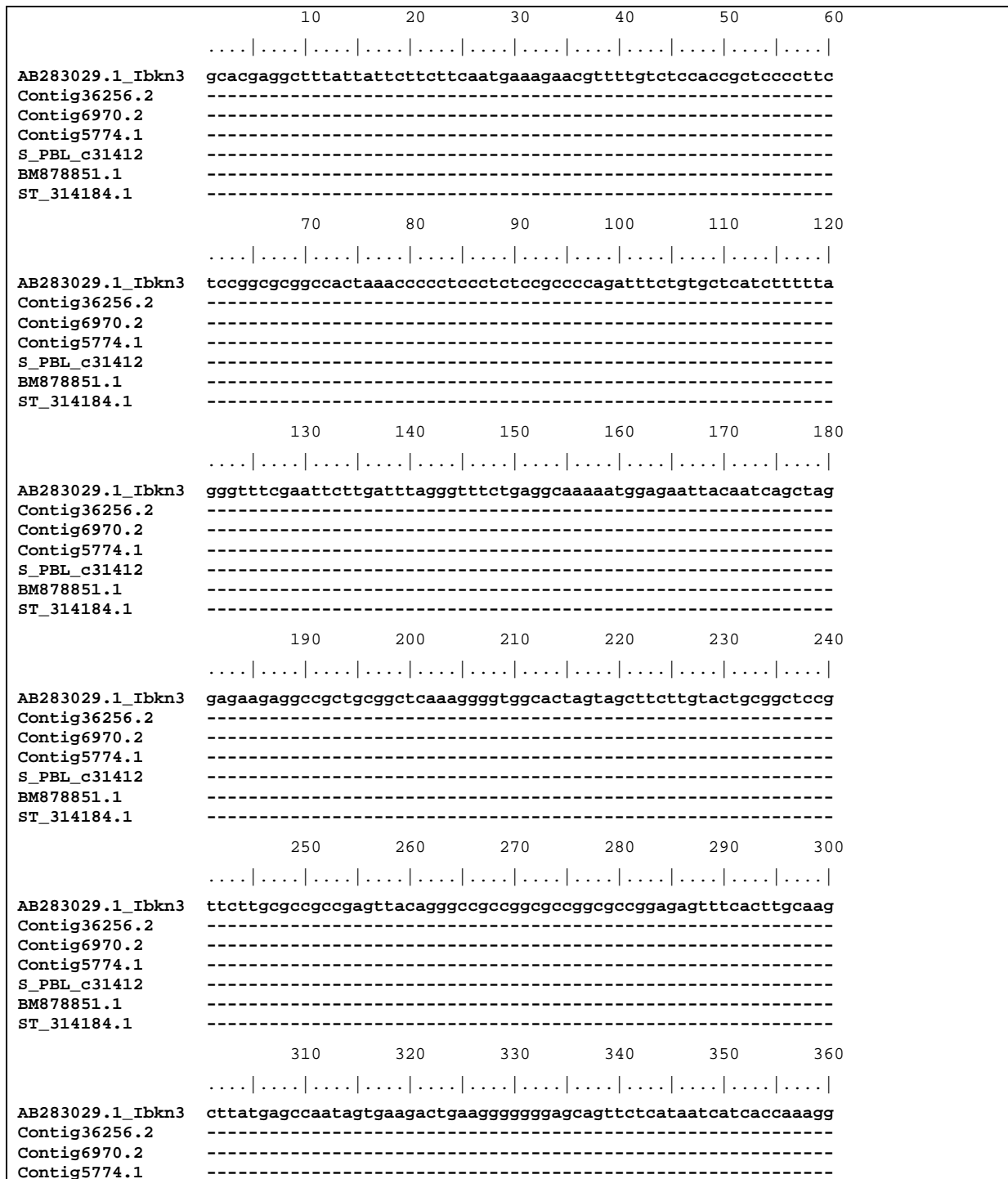
Figure 3.3 Alignment of Ibkn3-like sequences.
