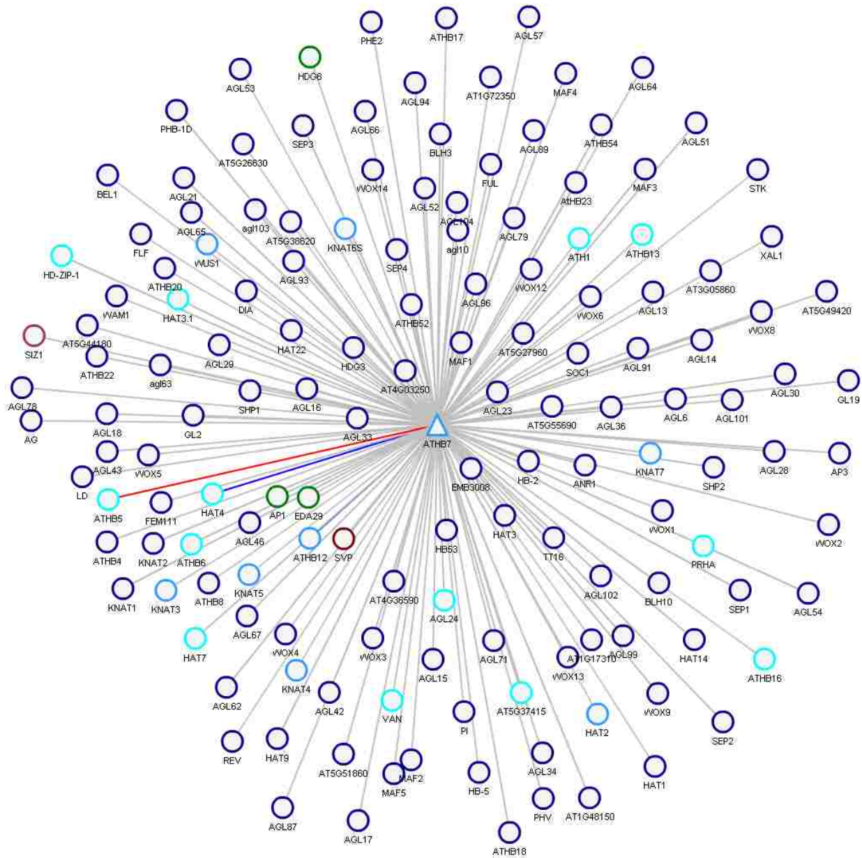
Figure 2.4. Interaction network of proteins predicted to interact with ATHB7 from Predicted Arabidopsis Interactome Resource tool ( http://www.cls.zju.edu.cn/pair/faces/home.xhtml ) ( http://www.cls.zju.edu.cn/pair/faces/searchinteraction.xhtml )
