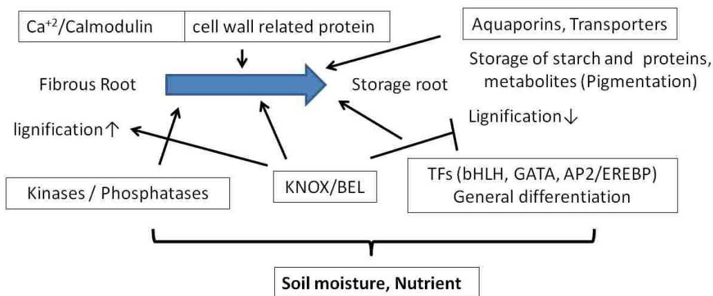
Figure 5.1. Hypothesis of proteins involved in storage root formation. TF=transcription factors. Calcium signaling is an important component in the onset of storage roots. Regulatory transcription factor might act as a network that influence both metabolic pathways (enzymes) as well as transport and allocation of secondary metabolites. Expression of Knox/BEL genes that act by possibly suppressing the lignification in a similar way to Arabidopsis , peach and poplar. Post-transcriptional modifications are involved in triggering the phase of fibrous to storage root and in response to the environment.
