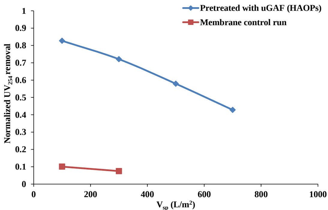
Figure 4.8 NOM removal (presented in \text{UV}_{254} ) from 50% LP water with or without \mu\text{GAF} pretreatment
