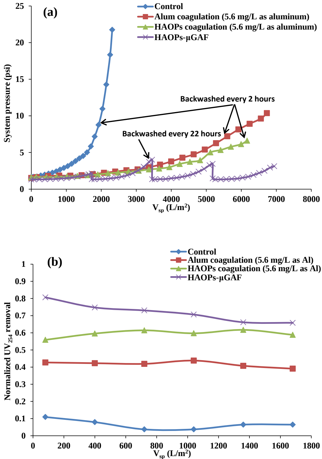
Figure 4.32 (a) Pressure increase profiles of four different approaches and (b) fractional removal of NOM (presented in UV 254 ) of four different approaches for treating LU water
