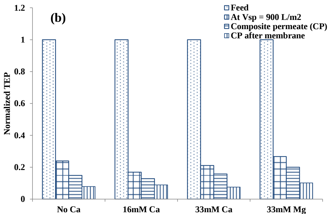
Figure 4.28 Sequential \mu GAF-membrane filtration permeate quality at different \text{Ca}^{2+}/\text{Mg}^{2+} concentration (a) UV 254 absorbance and (b) TEP concentration
