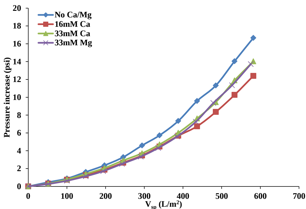
Figure 4.26 Bare membrane fouling when fed with 50% LP water of different \text{Ca}^{2+}/\text{Mg}^{2+} concentration. Total ionic strength fixed at 100mM.
