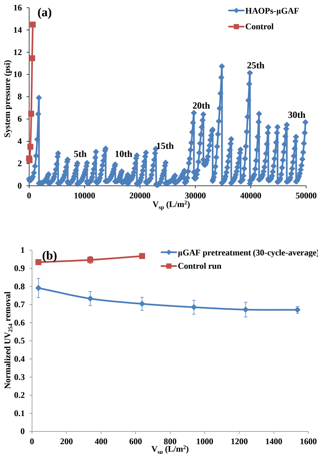
Figure 4.33 (a) Pressure increase profiles of the \mu GAF system during 30 sequential, 22-h filtration cycles and (b) average NOM removal (presented in UV 254 ) of permeate from \mu GAF system in each filtration cycle. A control run is presented as reference
