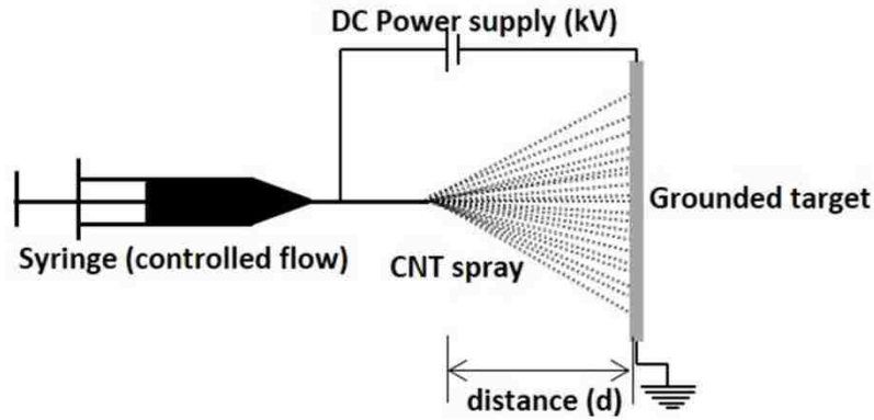
Figure 5-2: Schematic diagram of the electro spray deposition
