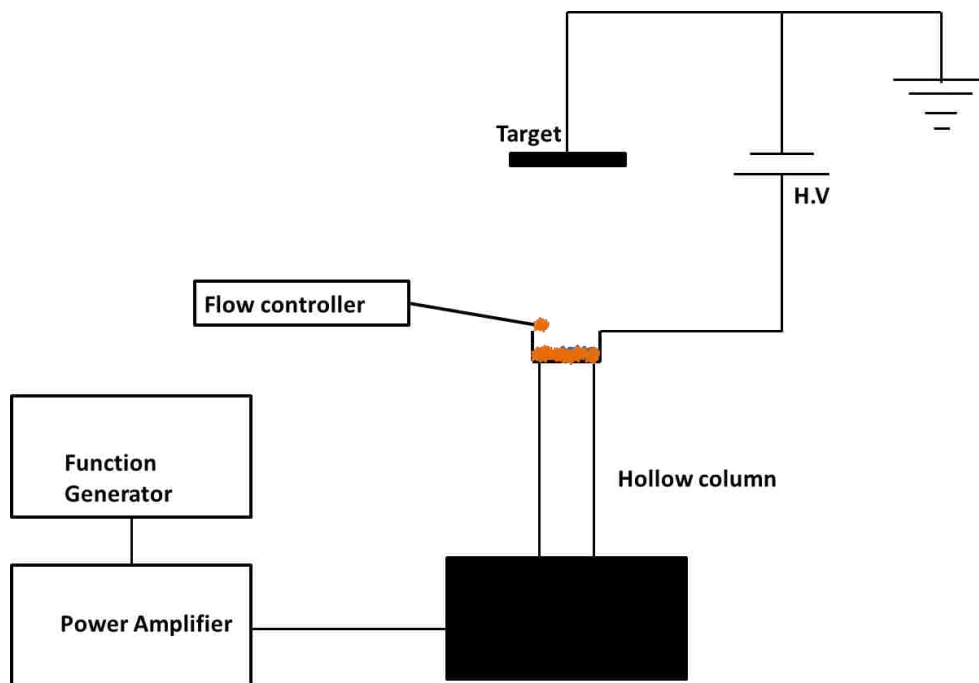
Figure 6-4: Schematic of electrostatic spraying with sound waves setup
