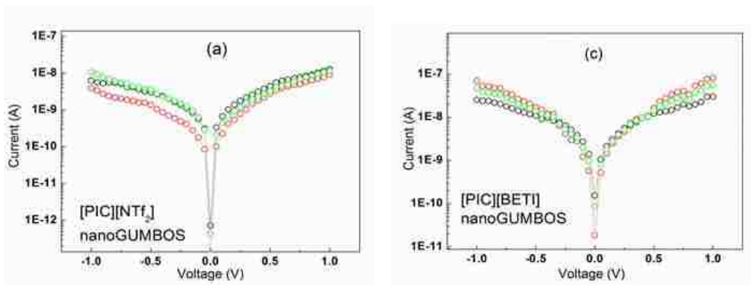
Figure 4-28: Log plot of Current-voltage (I-V) curves of [PIC][NTf 2 ] and [PIC][BETI] nanoGUMBOS obtained by conductive probe atomic force microscopy (CP-AFM) (Reprinted with permission from Springer [97]).
