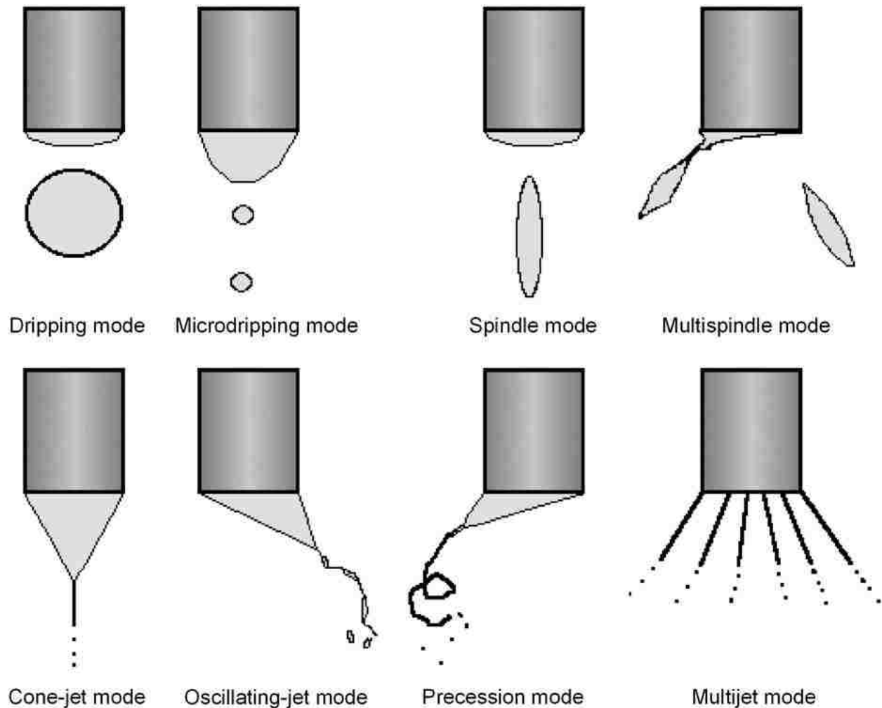
Figure 2-5: Various modes of electrospaying (Reprinted with permission from[42]. Copyright (2008) Elsevier)
