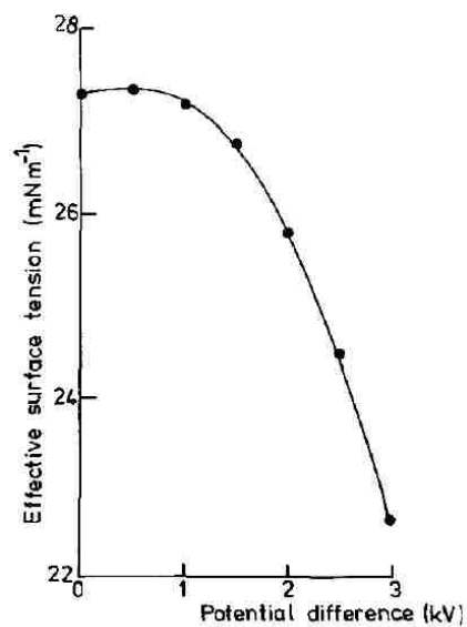
Figure 2-2: Surface tension as a function of applied potential (Reprinted with permission from[45]. Copyright (1987) Elsevier)
