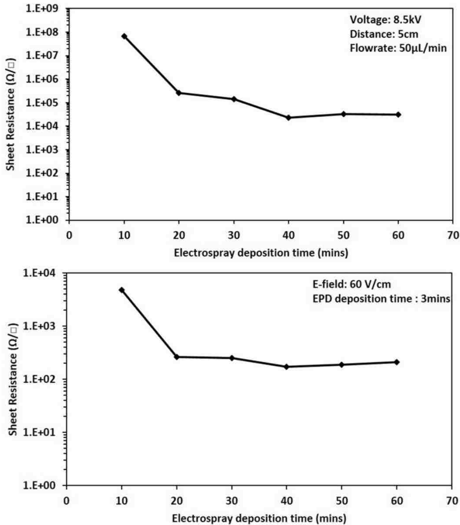
Figure 5-8: (a) Variation in sheet resistance of the electro sprayed CNT films as a function of deposition time from 10 min to 60 min, and (b) variation of sheet resistance values of the final CNT coating by EPD in relation to varying electro spraying deposition time from 10 min to 60 min (EPD was performed at a constant applied E-field of 60 V/cm with 3 min of deposition on the underlying CNT coating).
