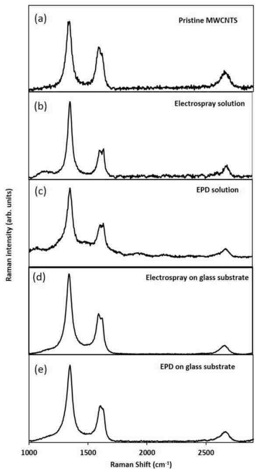
Figure 5-9: Raman spectra of (a) pristine MWCNTs, (b) acid refluxed and ultrasonicated CNT solution in ethanol, (c) ultrasonicated electrospay CNT-IPA for EPD, (d) electrospayed CNT coating on glass substrate, and (e) final CNT coating obtained by EPD. All of the spectra displayed signature Raman peaks of MWCNTs at 1336 \text{ cm}^{-1} , 1587 \text{ cm}^{-1} and 2648 \text{ cm}^{-1} wavenumber.
