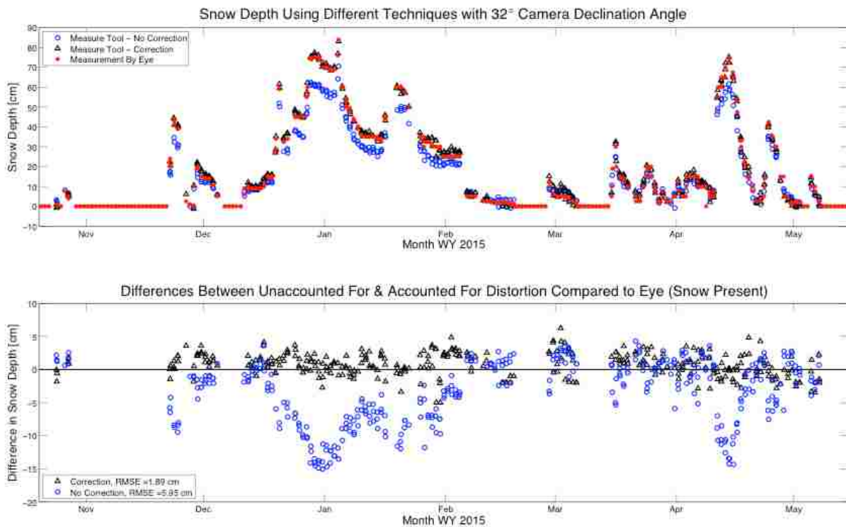
Figure 6: Evidence that this technique corrects for the perspective distortion, which can occur if only a single length per pixel value was used. For both the corrected and not corrected images 14 random calibrations were done and the mean was taken. The second plot shows the difference from eye for both techniques when there was snow. Large differences from an eye measurement occur when snow depth increases and distortion is not accounted for (Blue). The differences greater than 5 cm are systematic errors stemming from the methodology that used a single length per pixel.
