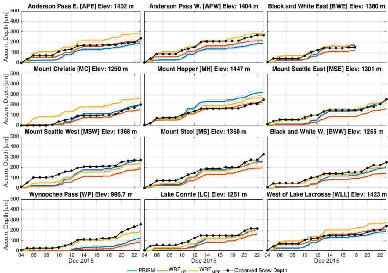
Figure 6: Accumulated snow depth between 4 and 23 December 2015 during the OLYMPLEX intensive observational period. Observed accumulated snow depth is shown in black and the ensemble mean of the simulated cumulative snowfall is shown in the thick colored line. Individual ensemble members are again shown in thin dotted lines.
