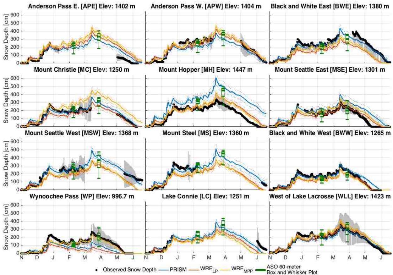
Figure 4: Snow depth time-series at all twelve independent measurement sites. Thick line represents the ensemble mean for PRISM, WRF_{LP} , and WRF_{MPP} while the thin dotted lines represent individual ensemble members. Black dotted lines with gray shading show the angle corrected snow depth measurements from the time-lapse camera network along with their relative uncertainty. Green box and whisker plots show the distribution of values from within a square 60-meter area around the snow depth pole. The minimum and maximum values of the box and whisker plot show the bottom 10% and top 90% of the snow depth values within the 60-meter bounding box, respectively.
