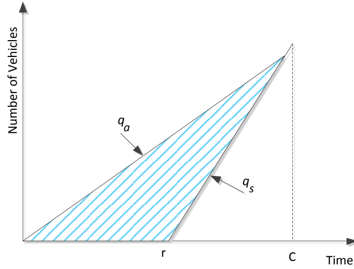
Figure 3-5: Arrival and Departure Curves with Uniform Arrival Rate
