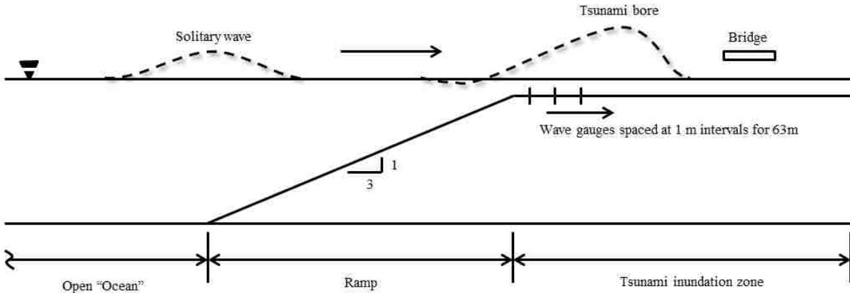
Figure 6-6: Schematic of the OpenFOAM™ Model
