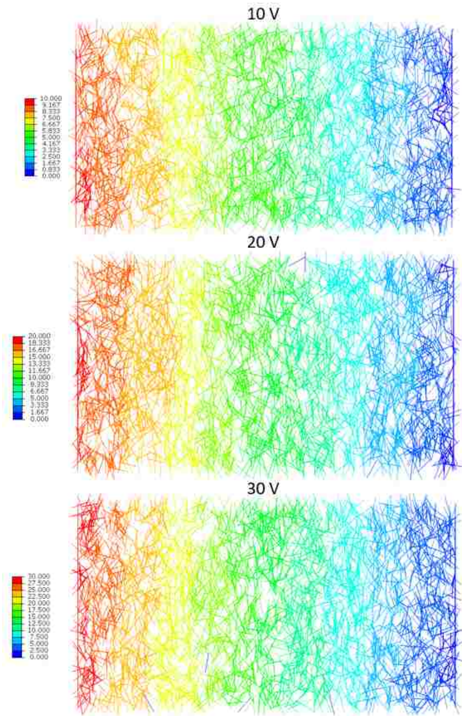
Figure 5.15: Voltage Variations
