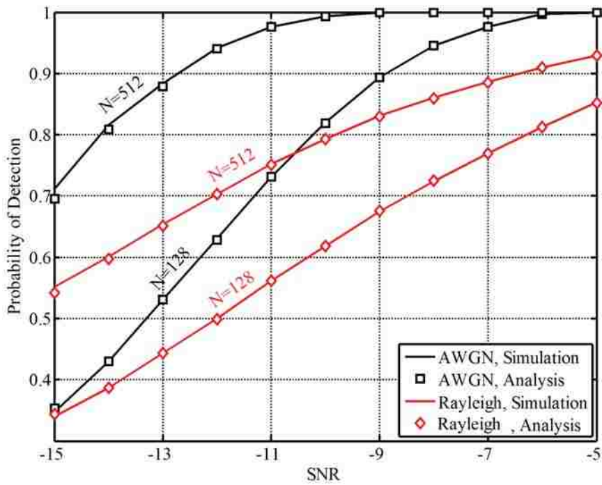
FIGURE 2.1. p_1 versus SNR for Rayleigh and AWGN channel, doubinary signaling, and different values of N
