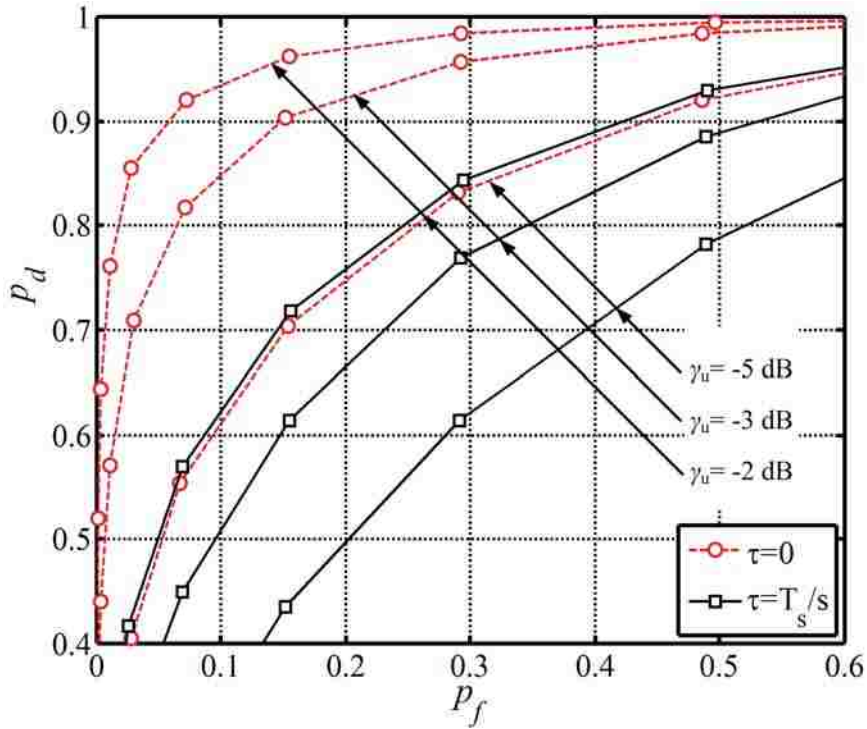
FIGURE 4.5. ROC for (511, 304)-BCH code, CRC-8, 16-QAM and 64-QAM for the SU and the PU, \gamma_s = 5\text{dB} , different \gamma_u , and \tau = 0, T_s/2 .
