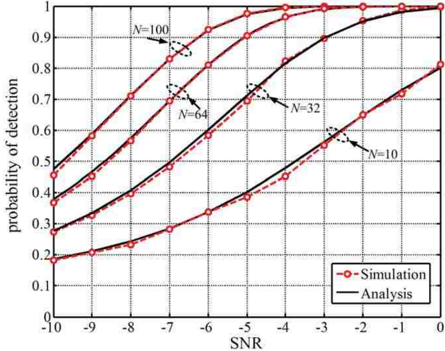
FIGURE 5.3. Probability of detection vs. SNR using T_{ge} for M = 4, L = 3, P_0 = 0.1, \theta_{max} = \pi/4 and different values of N .
