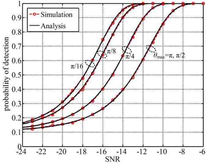
FIGURE 5.6. Detection probability vs. SNR using T_{gc}(L) for different values of \theta_{\max} , with M = 4 , L = 3 , P_0 = 0.1 , N = 1024 .
