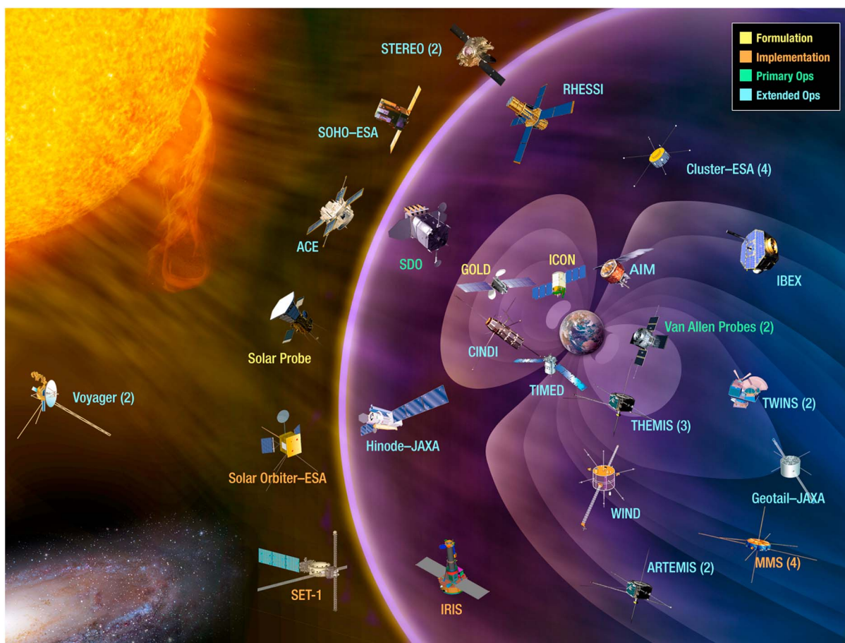
Figure 1. Artist's rendition of the Sun-Earth space environment (not to scale), with NASA's Heliophysics System Observatory overlaid. Image courtesy of NASA.
