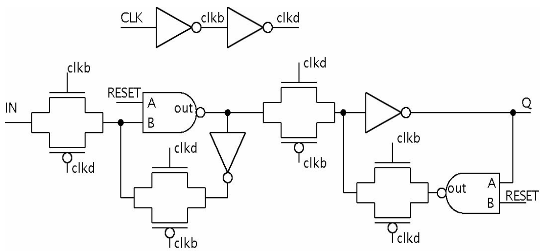
Figure 1.2: D Flip-Flop circuit diagram of a phase/frequency detector (PFD).
