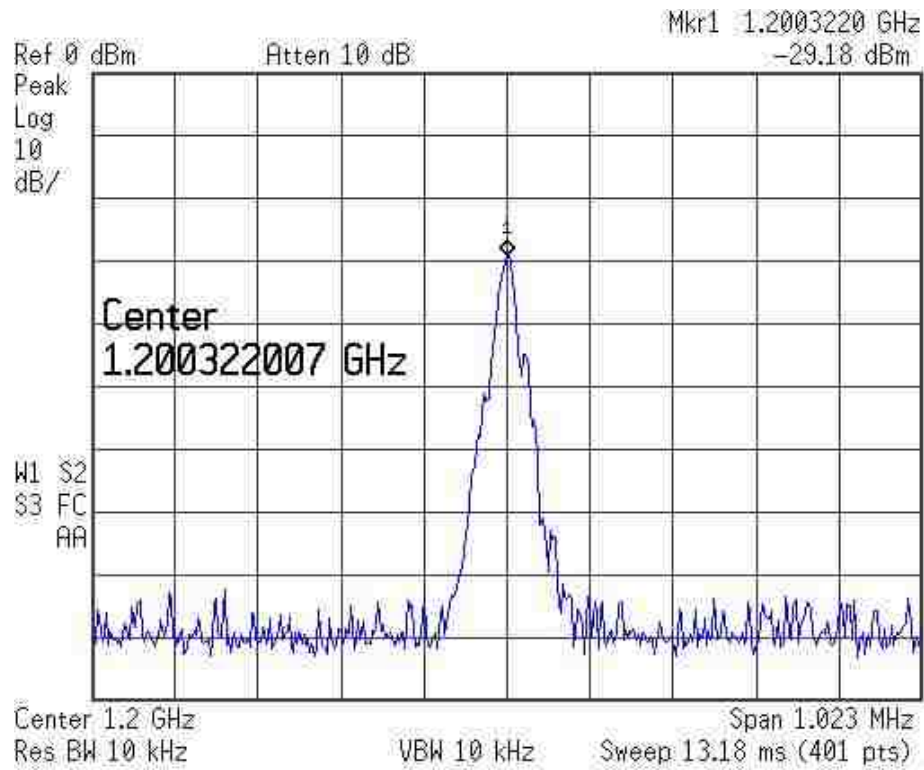
Figure 4.16 (a): Power spectrum density measurement without hot carrier effect. Note: The Y axis scale is -10dB per grid from Ref 0 dBm.
