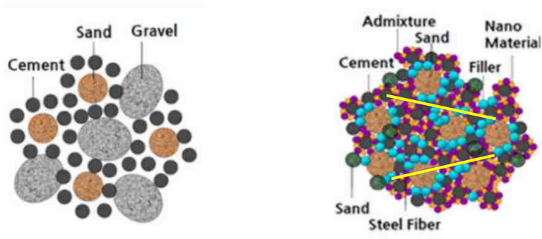
Appendix Figure A.2. Microstructure composition of conventional concrete (left) and UHPC (right).
