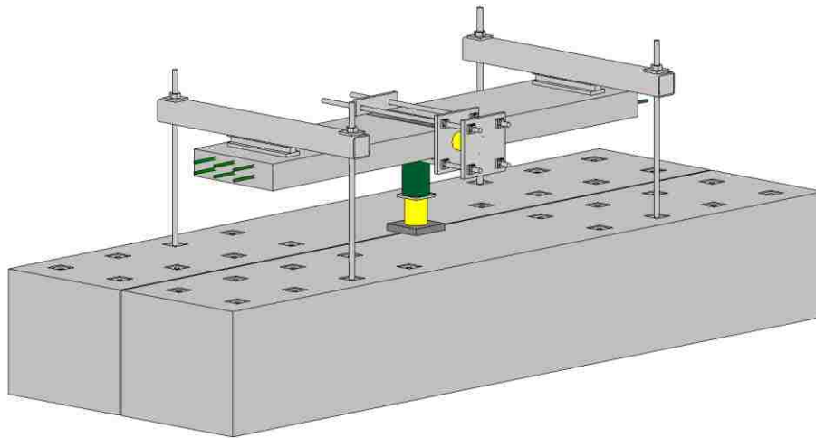
Figure 5.9. 3D model of the simulated deck test apparatus.
