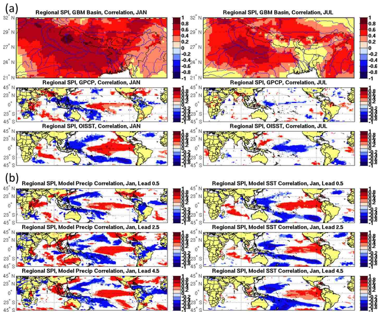
Figure 2.3. (a) Observed area-average SPI correlations with observed rainfall (significant at the p < 0.10 level) at each point over (top) the GBM basin, with large-scale precipitation from (middle) GPCP and (bottom) SST. Both (left) January and (right) July are illustrated. (b) The observed January area-average SPI correlations with the NMME seasonal forecasts (significant at the p < 0.10 level) for (left) precipitation and (right) SST at lead times of (top) 0.5, (middle) 2.5, and (bottom) 4.5 months. Note the similarity of tropical precipitation and SST signals with those in (a).
