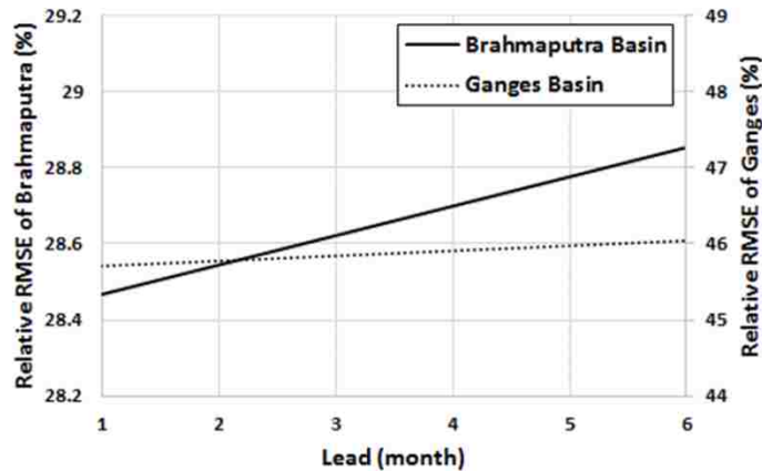
Figure 2.5. Relative RMSE (normalized by SGF) trend of NMME precipitation forecast (during 1982–2012) over the entire Ganges and Brahmaputra basin as a function of lead time (months). Note that the trend is idealized as a linear regression mainly to observe sensitivity to lead time.
