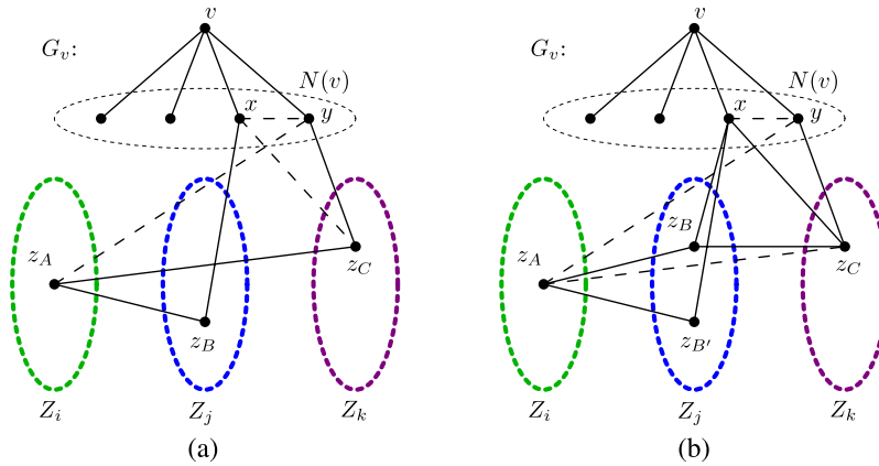
Fig. 6. For the proofs of: (a) Lemmas 3.4 and 3.6; (b) Lemmas 3.5 and 3.7 (edges that may or may not exist are shown dashed).
