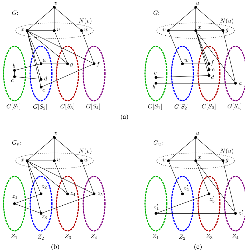
Fig. 4. (a) The same graph shown in two different ways (with respect to vertices v and u ); (b) the graph G_v ; (c) the graph G_u .
