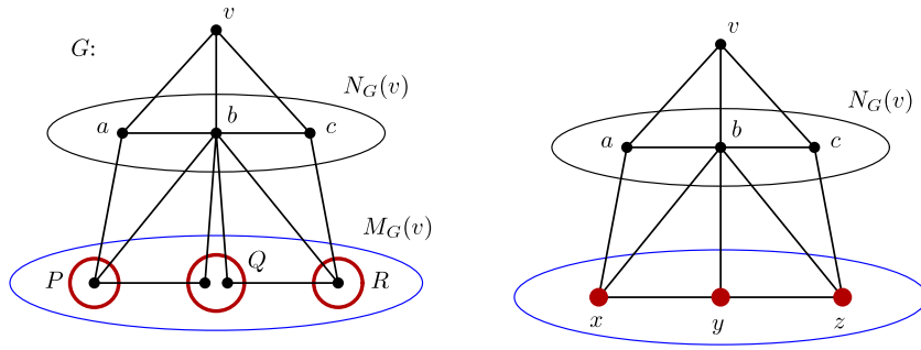
Fig. 3. Shrinking each partition set into a single vertex may lead to error.
