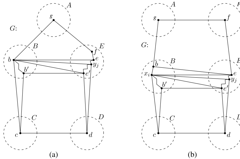
Fig. 5. For the proof of Corollary 3.1; (a) for the case of a house ( x_i coincides with b ); (b) for the case of a domino.
