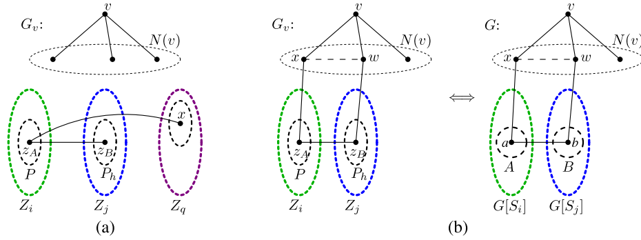
Fig. 8. For the proof of Theorem 3.1.
