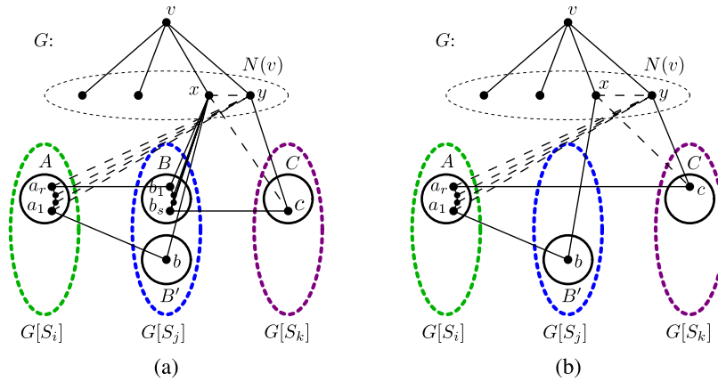
Fig. 9. For the certificate computation at Step 4.2.
