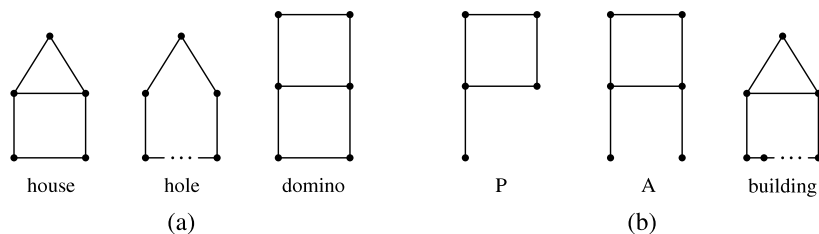
Fig. 1. (a) The forbidden graphs for the class of HHD-free graphs. (b) The graphs ‘P’, ‘A’, and the building.
