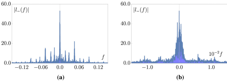
Fig. 18. Power spectrum for the chaotic attractor (spin dynamics in Fig. 14) at \delta = 0.100, W = 0.055 . It is a continuum without any reflection symmetry about the f = 0 axis. The spectrum has several peaks. The most prominent of those is located at the origin. In (b), we magnify the region near f = 0 by a factor of 10^2 to accentuate the peak there.
