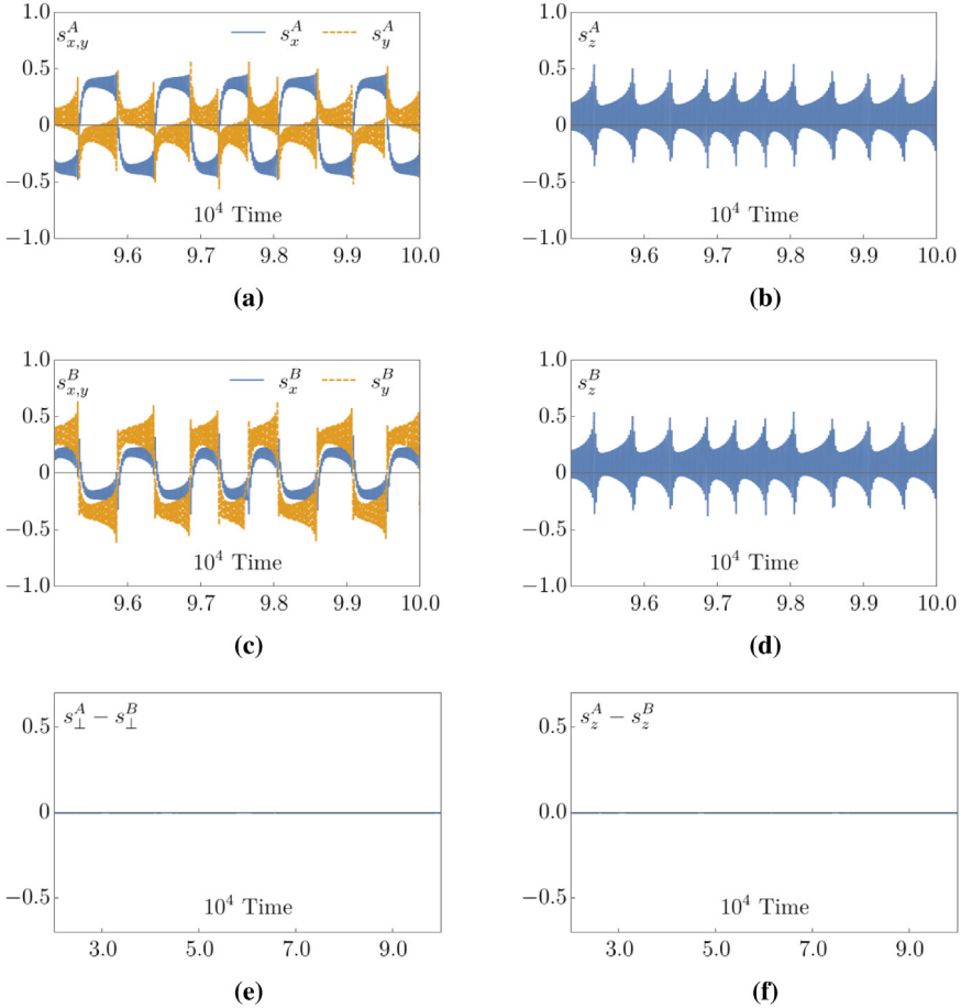
Fig. 21. Dynamics of s^A and s^B in the synchronized chaotic phase at \delta = 0.080, W = 0.055 with the same conventions as in Figs. 6 and 14. The time dependence of the spin components are markedly different from that in other phases. The chaotic nature of the spin dynamics, however, is apparent from (a), (b), (c) and (d). At large times, the differences between s_{\perp}^A and s_{\perp}^B , and s_z^A and s_z^B being equal to zero is due to the \mathbb{Z}_2 symmetry of the chaotic attractor. The reflection symmetry about f = 0 axis in the spectrum in Fig. 24 is due to the above symmetry.
