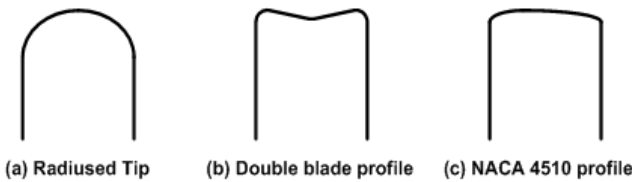
Figure 1. The three different vane tip geometries [4].
