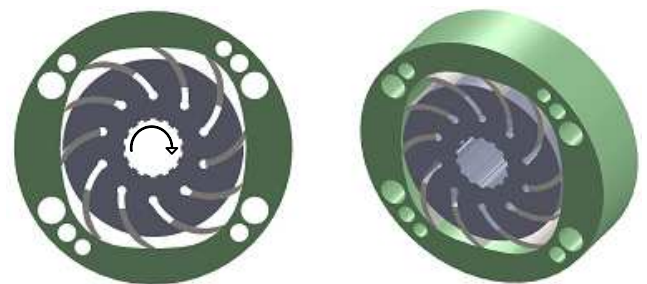
Figure 4. Forward curved vane geometry for balanced hydraulic vane machine.
