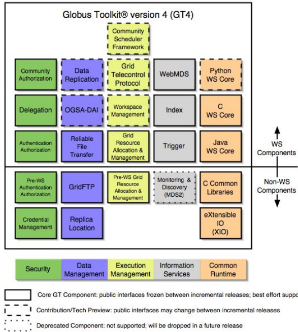
FIGURE 3.1: Globus ToolKit 4.0 Architecture
