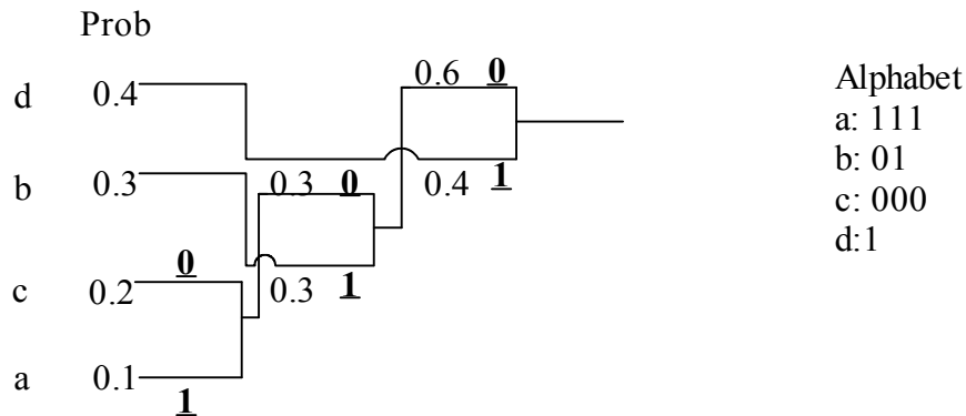
Figure 2.2. Huffman Code Construction. From this example the message dccb would be coded as 11000000111101.
