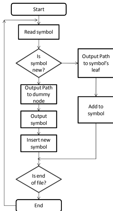
Figure 5.4. Encoding flowchart
