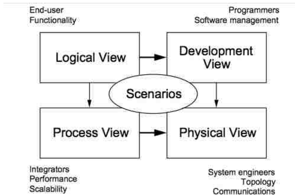
FIGURE 2.4: Krutchen’s 4+1 View Model of Software Architecture [Kru95]
