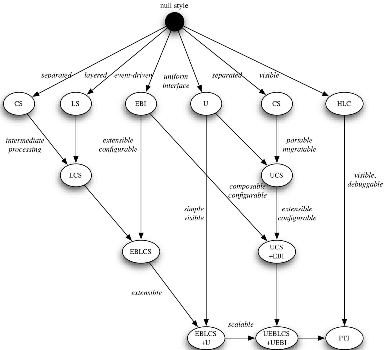
FIGURE 5.1: PTI derivation by style constraints
