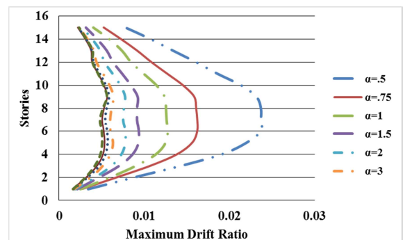
Figure 17. Maximum drift of the 15 stories building.
