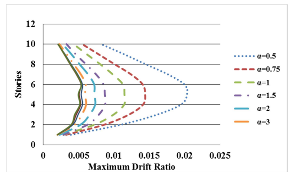
Figure 16. Maximum drift of the 10 stories building.
