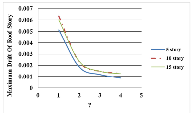
Figure 13. Maximum drift of the highest story versus \gamma .
