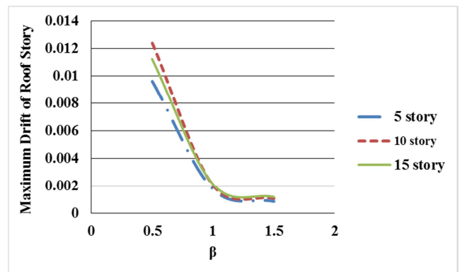
Figure 8. Maximum drift of the highest story versus \beta .
