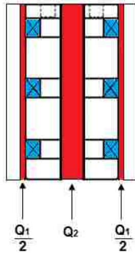
Figure 4.5. Flow rates in each flow passage of the MR valve and the center orifice of the passive valve
