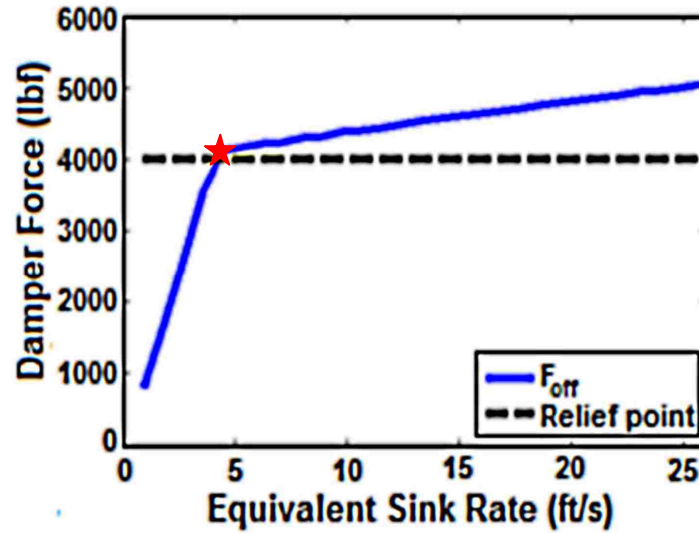
Figure 4.21. MR passive relief valve damper force is designed to open around an equivalent sink rate of 4.4 ft/s (1.34 m/s) for MTS ramp tests using the spiral wave spring with a stiffness of 59.8 lb f /in and the coil spring using a stiffness of 47.5 lb f /in
