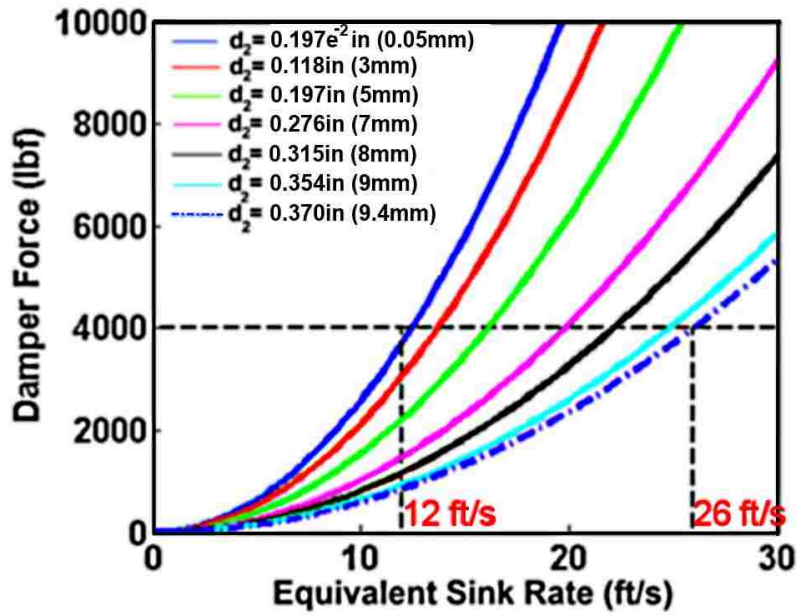
Figure 4.6. Damper force (in \text{lbf} ) versus sink rate (in \text{ft/s} ) for different orifice diameters, d_2
