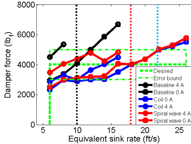
Figure 5.5. Maximum achievable equivalent sink rate of the MR landing gear dampers within a force error bound of \pm 1000 \text{ lb}_f (the drop mass was 1283 lbs)
