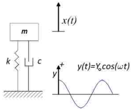
Figure 1.5. A particular helicopter seat and occupant system represented using a single-degree-of-freedom system (SDOF system)
