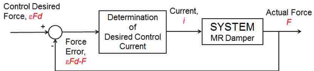
Figure 5.6. Block diagram of the bang-bang current control algorithm used for single MR landing gear damper drop tests
