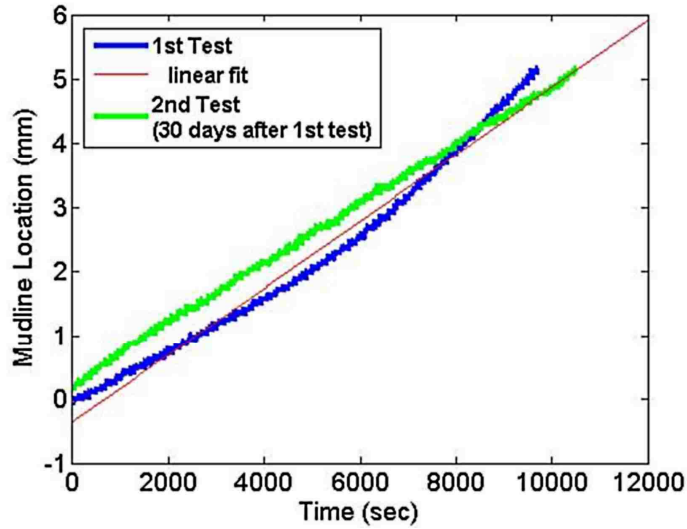
Figure 2.6. Settling rates of mr83282-Ie (containing 6-10 \mu m particles at 80 wt% concentration). Testing was performed one month apart.
