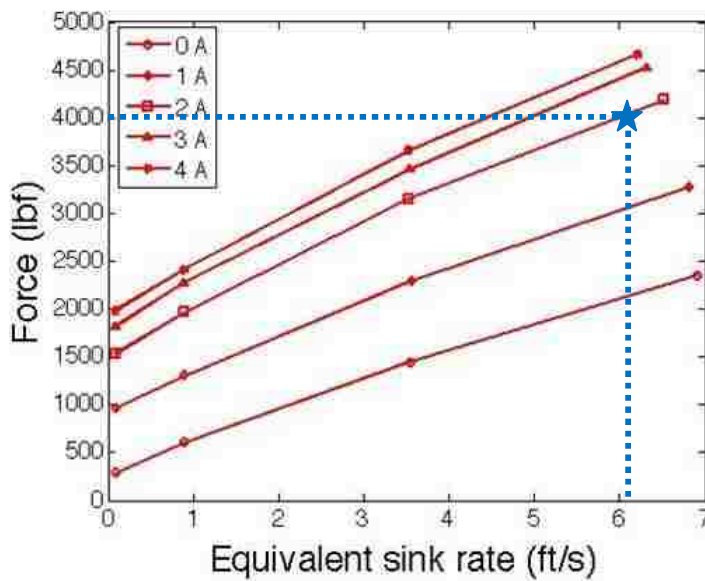
Figure 4.20. MTS machine capability of reaching equivalent sink rates of about 6.2 ft/s (or 1.89 m/s) while maintaining a stroking load of 4000 lbf in the landing gear damper at the University of Maryland
