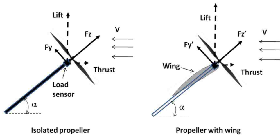
FIGURE 4.10: Differences in forces produced by a propeller in non-axial flow, with and without wing
