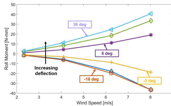
FIGURE 6.10: Torque generated by a single wing tip in forward flight
