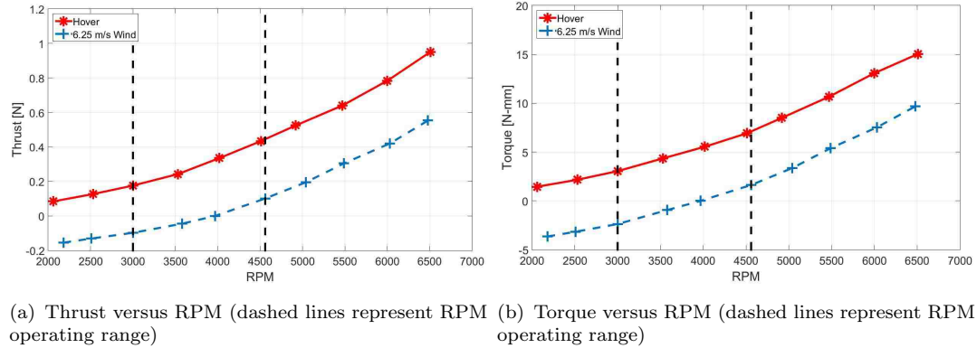
FIGURE 6.7: Original roll control performance plots with GWS 6x5 proprotor
