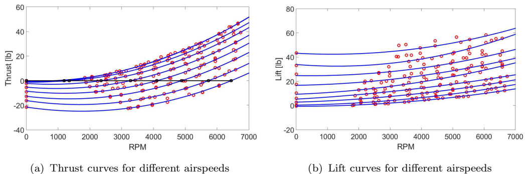
FIGURE 7.6: Polynomial curve fits of test data
